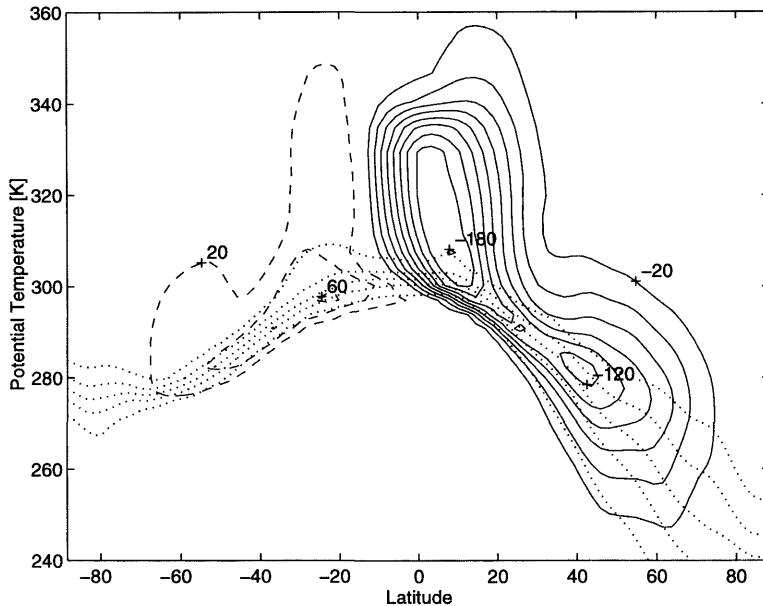
Fig. 1. The mean meridional mass transport in isentropic coordinates, as obtained from the January climate of an R30, 14 level atmospheric general circulation model. The contour interval for the streamfunction is 2 \times 10^{10} kg/s. The five dotted lines represent the probability distribution (the 10%, 30%, 50%, 70%, and 90% isolines) for the surface potential temperature. (Surface potential temperature is above the 10% isoline 10% of the time, etc.).
