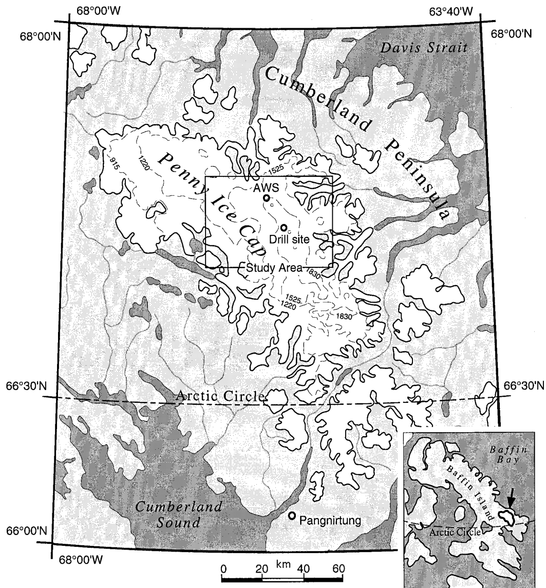
Fig. 1. Location map of the Penny Ice Cap, Cumberland Peninsula, southern Baffin Island. The location of the automatic weather station (AWS) and ice core drilling site are shown. Contour intervals in meters.
