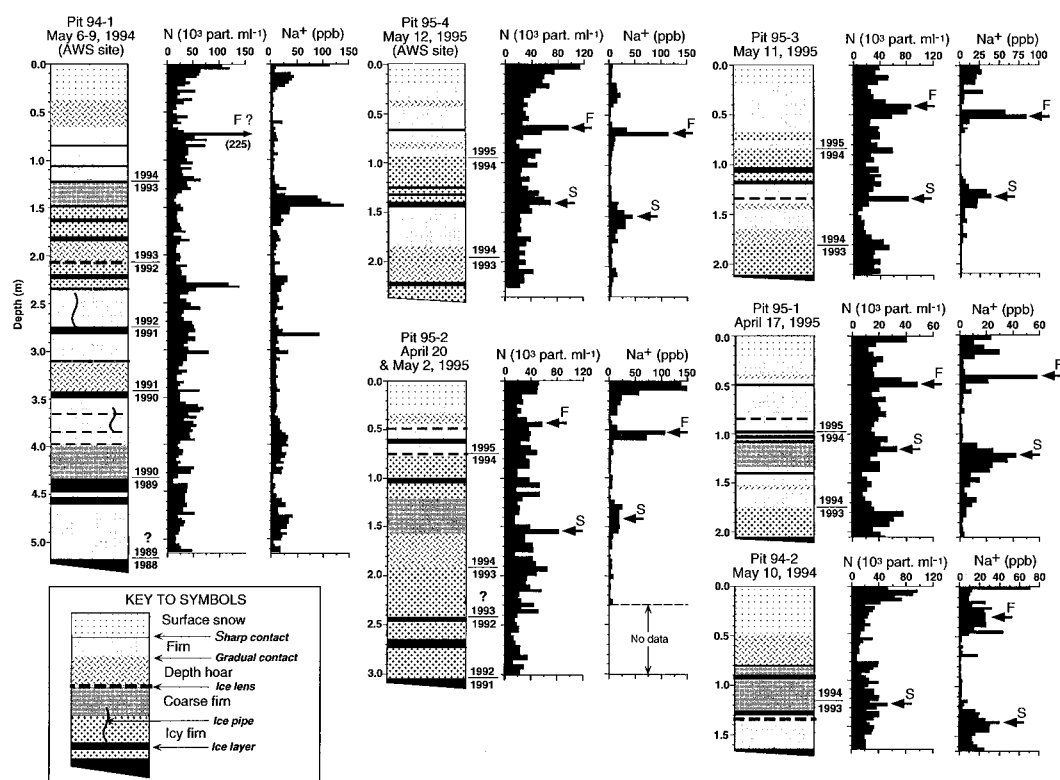
Fig. 3. Physical stratigraphy and profiles of dust ( N ) and Na^+ concentration in six snowpits excavated at the summit of the Penny Ice Cap. Accumulation years are delineated by the end of the ablation season, as discussed in text. Arrows with labels indicate the inferred seasonal input timing for Na^+ and dust peaks (S = Spring; F = Fall).
