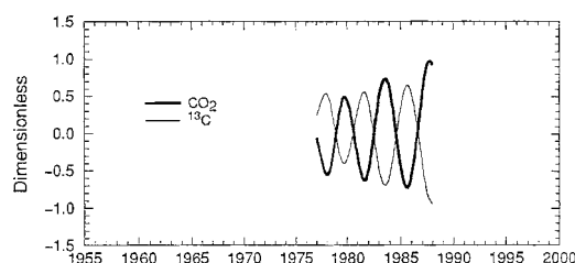
Fig. 12. Bivariate SSA reconstruction of the leading (QQ) mode of shared interannual variability of Mauna Loa \text{CO}_2 and the average of seasonally adjusted \delta^{13}\text{C} series from Mauna Loa and the South Pole.
