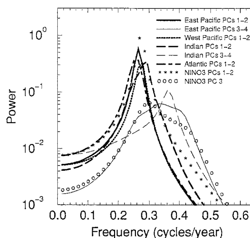
Fig. 8. Maximum-entropy spectra of leading principal components (PCs) from bivariate SSAs of detrended, deseasonalized Mauna Loa CO 2 series with tropical SSTs between 20°S and 20°N, in the eastern Pacific (150°W–80°W), western Pacific (120°E–150°W), Indian (35°E–120°E), and Atlantic (80°W–15°E) Oceans, and in the Niño-3 region of the eastern Pacific (5°S–5°N, 150°W–90°W). The analyses are all carried out over the 1958–1993 interval; see legend in figure.
