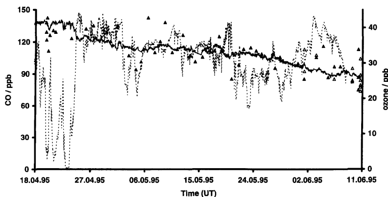
Fig. 3. Time series of carbon monoxide and ozone mixing ratios determined by different methods and at different locations. Solid line: in-situ measurements (Gruvebadet), solid triangles: canister samples (Zeppelin Mountain), open triangles: canister samples (Gruvebadet), dashed line: ozone (airport). Institut für Umweltphysik, Heidelberg, Germany (H. Lorenzen-Schmidt personal communication).
