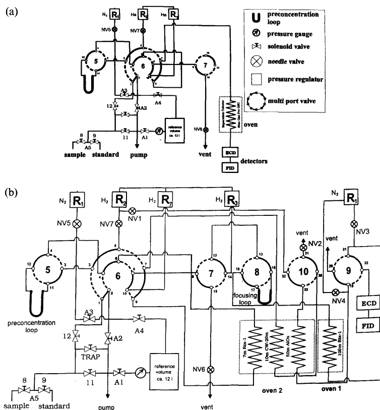
Fig. 2. (a,b) Schematic drawings of the gas chromatographic set-ups used in this study, symbols used consistently for both figures.
