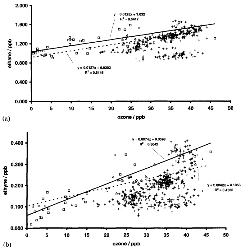
Fig. 7. (a–d) Plots of ozone versus selected NMHC including linear correlations. triangles, dashed line: minor depletion period (2 May 00:00–5 May 23:59), squares, solid line: major ozone depletion period (18 April 00:00–24 April 23:59), crosses: normal ozone.
