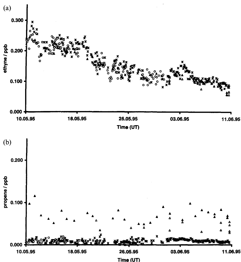
Fig. 4. (a,b) Comparison of the ethyne and propene mixing ratios determined by different methods and at different locations. Stars: GC1 in-situ measurements (Gruebadet), circles: GC2 in-situ measurements (Gruebadet), solid triangles: canister samples (Zeppelin Mountain), open triangles: canister samples (Gruebadet).
