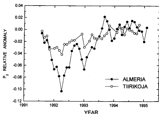
Fig. 7. Anomaly in atmospheric integral transparency coefficient p_2 , at Almería and Tiirikoja. The anomaly is represented in relative terms, showing the ratio between the reduction in p_2 and the seasonal pattern obtained for pre-eruption conditions at both places.
