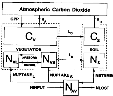
Fig. 2. The terrestrial ecosystem model (TEM). The state variables are: carbon in vegetation ( C_V ); structural nitrogen in vegetation ( N_{VS} ); labile nitrogen in vegetation ( N_{VL} ); organic carbon in soils and detritus ( C_S ); organic nitrogen in soils and detritus ( N_S ); and available soil inorganic nitrogen ( N_{AV} ). Arrows show carbon and nitrogen fluxes: GPP, gross primary productivity; R_A , autotrophic respiration; R_H , heterotrophic respiration; L_C , litterfall carbon; L_N , litterfall nitrogen; NUPTAKE_S , N uptake into the structural N pool of the vegetation; NUPTAKE_L , N uptake into the labile N pool of the vegetation; NRESORB , N resorption from dying tissue into the labile N pool of the vegetation; NMOBIL , N mobilized between the structural and labile N pools of the vegetation; NETNMIN , net N mineralization of soil organic N; NINPUT , N inputs from the outside of the ecosystem; and NLOST , N loss from the ecosystem. (From Melillo et al., 1993, reprinted with permission from Nature 363, 234–240, © 1993 MacMillan Magazines Limited.)
