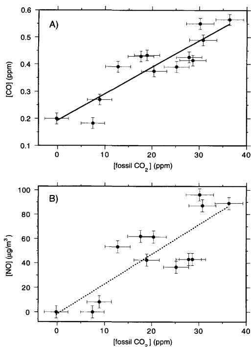
Fig. 4. (A) Correlation between the CO concentration and the concentration of fossil CO 2 , derived in the present work. There is good correlation. The slope of the regression line corresponds with CO: fossil CO 2 = (0.0098 \pm 0.0014):1 . The intercept ( 0.19 \pm 0.03 ppm) agrees with what is to be expected for continental background conditions. (B) Correlation between the NO concentration (in µg/m³) and the concentration of fossil CO 2 . Correlation is reasonable.
