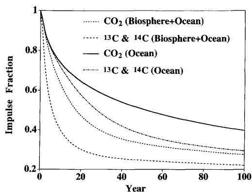
Fig. 7. Model-estimated atmospheric response to a pulse input of \text{CO}_2 and \delta^{13}\text{C} and \Delta^{14}\text{C} . In addition to the ocean, the terrestrial biosphere and the soil will also absorb the carbon. Therefore, the figure shows the response to a pulse input with and without biospheric reservoirs. The amount of pulse was injected into a pre-industrial constant atmosphere.
