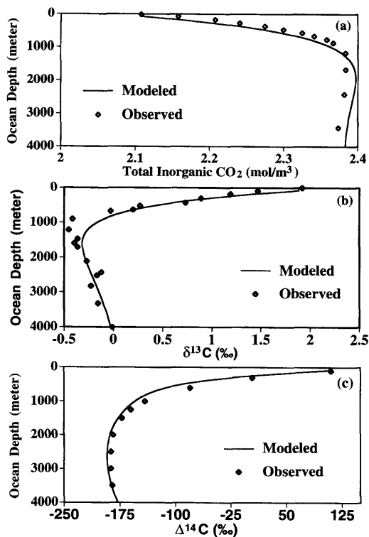
Fig. 5 Comparison of the model-estimated (a) total inorganic carbon (mol/m 3 ) (b) ^{13}\text{C} of dissolved inorganic carbon (‰) and (c) bomb-produced ^{14}\text{C} (‰) in the ocean with the observed data. The observed data in Figs. 5a, b, c are global averages of the GEOSECS data taken from Takahashi et al. (1981), Kroopnick (1985), and Shaffer and Sarmiento (1995), respectively.
