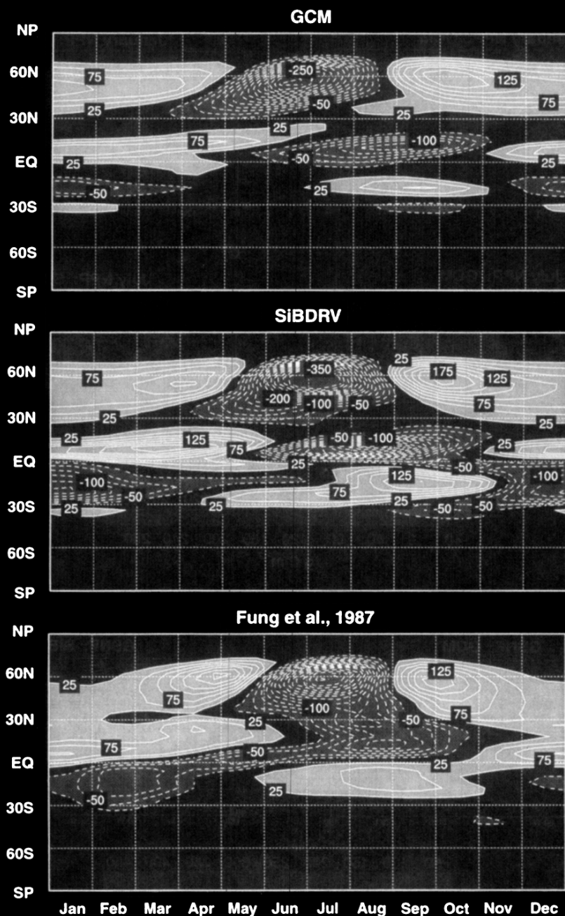
Fig. 3. Zonal total net flux of carbon ( 10^9 kg C month ^{-1} per 4^\circ latitude strip) from the land surface to the atmosphere by latitude and month of the year (a) as simulated by SiB2 in the GCM; (b) as simulated by SiBDRV; and (c) as calculated from the published estimates of Fung et al. (1987). The contour interval in all three panels is 25 \times 10^9 kg C month ^{-1} per 4^\circ latitude strip, with dark hatching for values above 50 and light hatching for values below -50 . For clarity, the zero contour has been omitted.
