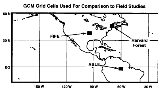
Fig. 5. Locations of 3 GCM grid cells used to compare the simulated carbon fluxes to observational data.
