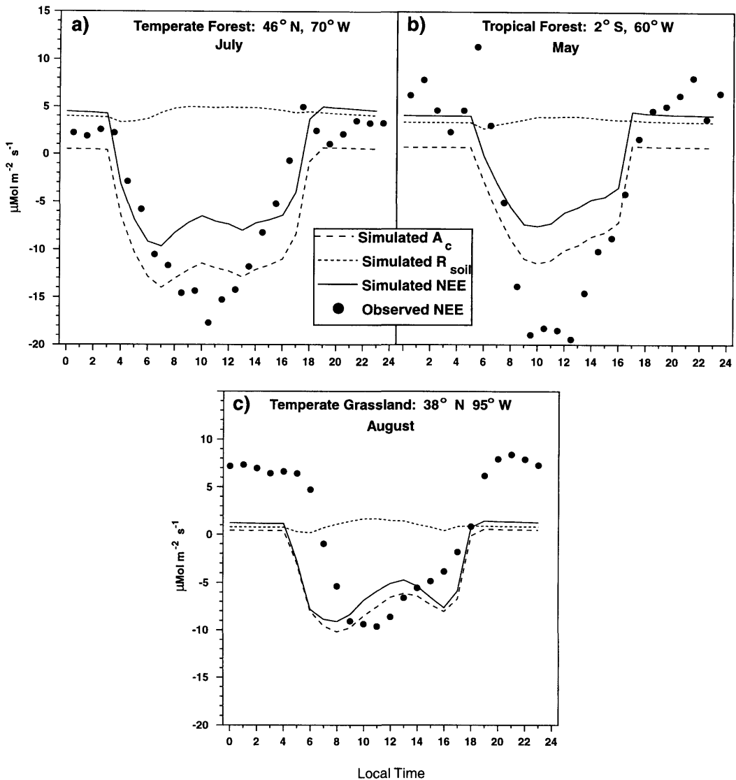
Fig. 7. Simulated monthly mean diurnal cycle of net canopy carbon assimilation ( A_c ), soil respiration ( R_{soil} ), and net ecosystem exchange (NEE), all in \mu\text{Mol m}^{-2} \text{ s}^{-1} , at the 3 locations indicated in Fig. 5, for various months in the final year of the GCM simulation. The net flux derived from eddy correlation measurements is indicated for comparison.
