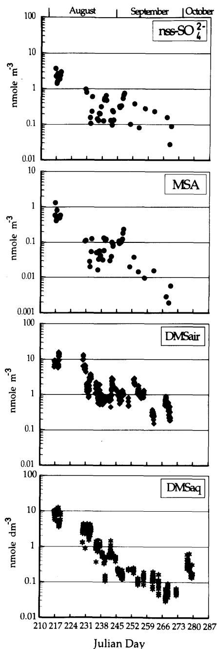
Fig. 2. Temporal distribution of seawater DMS, atmospheric DMS, and submicrometer aerosol MSA and \text{nss-SO}_4^{2-} in the "marine biogenic" sub population between August and October, 1991. All values are at STP. Between Julian Day 230 to 273 sampling was performed in the pack ice area.
