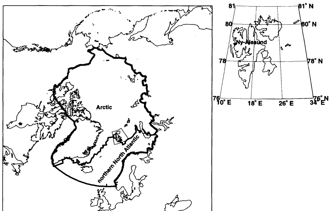
Fig. 1. The geographical position of the measuring site. The location of Ny-Alesund ( 78^{\circ}54' \text{N} , 11^{\circ}53' \text{E} ) is shown in the insert. In this work, the term "northern North Atlantic" is defined as the ice-free Atlantic north of 60^{\circ} \text{N} , as indicated in the overview chart. The area defined as "Arctic" is also shown in the main map.
