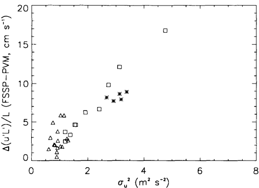
Fig. 3. Comparison of streamwise liquid water flux errors ( \Delta(u'L'/\overline{L}) ) with gustiness (streamwise wind variance, \sigma_u^2 ) during "a" events ( r^2 = 0.85 ). Note that the triangles represent the majority of the data; 1 May (asterisks) and 12 May (squares) data display the largest wind ramming errors.
