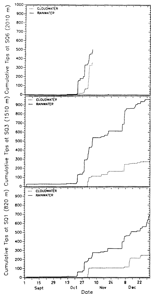
Fig. 3. Precipitation and cloudwater deposition at SQ1, SQ3, and SQ6 during the fall of 1987. Each tip of the rain gauge corresponds to 0.25 \text{ mm} of precipitation; each tip of the cloudwater gauge corresponds to 0.46 \text{ mm} of deposited cloudwater.
