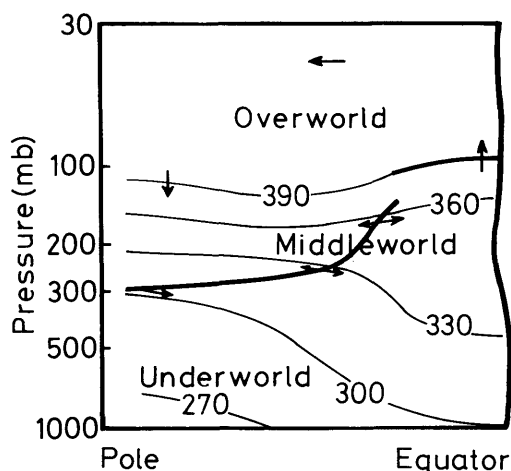
Fig. 1. A schematic view of the atmosphere as a function of latitude (pole-equator) and height (surface - 24 km). The tropopause is marked by a thick line, and isentropes every 30 K from 270–390 K by thin lines. The arrows indicate some transports. The equatorial boundary is defined by the zero PV contour.
