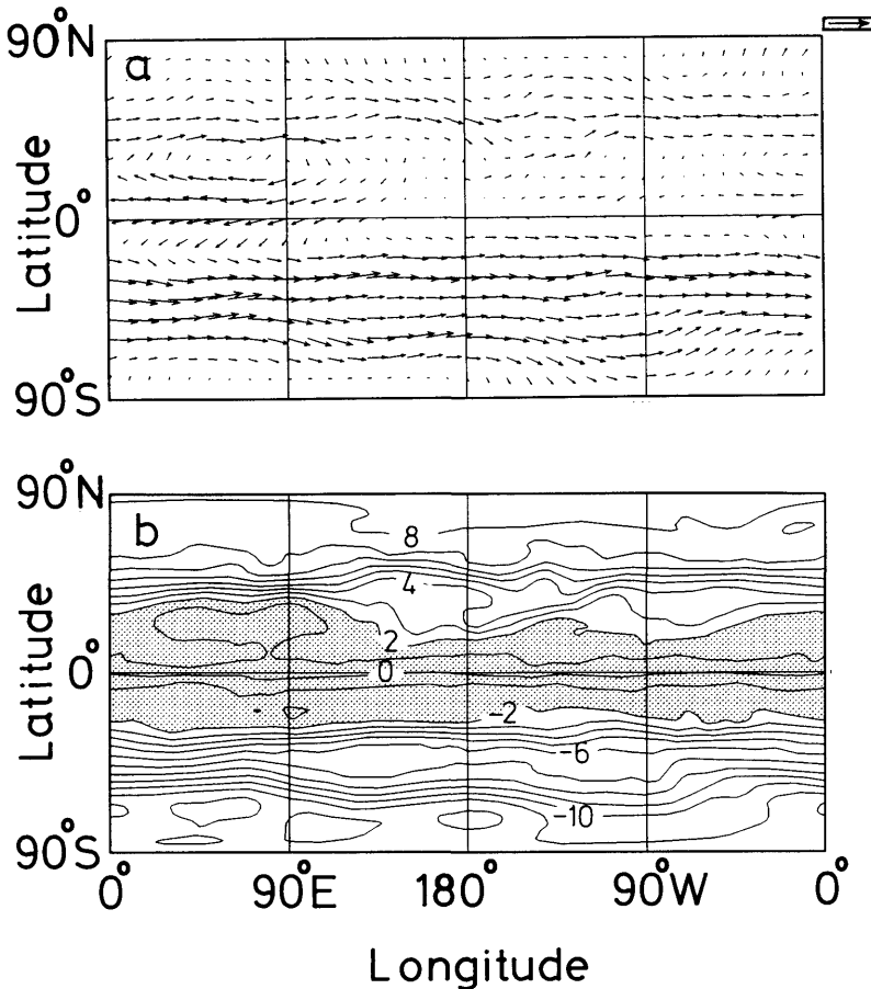
Fig. 4. Mean fields on the 360 K isentropic surface for August 1988. (a) \bar{v} with the arrow at the top right corresponding to 50 ms -1 . (b) \bar{P} with contour interval 1 PVU and values between -2 PVU and +2 PVU shaded.
