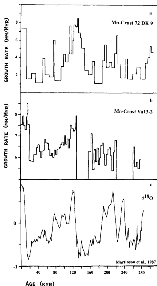
Fig. 1. Growth rates of Mn-crusts 72 DK 9 (a) and VA 13-2 (b) derived by applying a constant flux model on the Th-230 depth profile, against age (from Eisenhauer et al., 1990). (c) Generalized \delta\text{O}-18 chronostratigraphy after Martinson et al. (1987).
