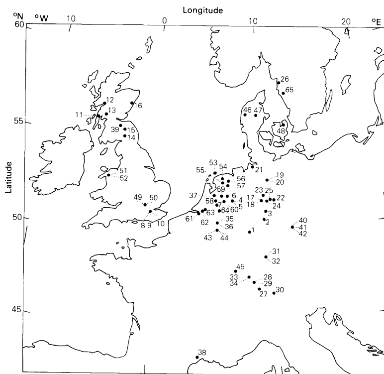
Fig. 1. Location of the case study sites. For references see Table 1.
