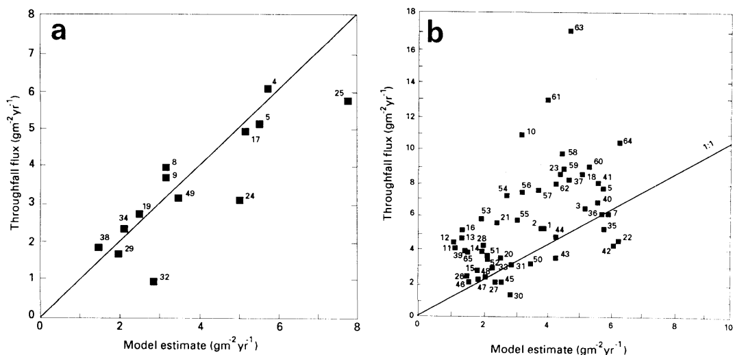
Fig. 3. (a) Sulfur flux onto the floor in 13 deciduous stands as a function of the total sulfur deposition calculated by the RAINS-EMEP model. (b) Sulfur flux onto the forest floor in 52 conifer stands as a function of total sulfur deposition calculated by the RAINS-EMEP model. For references see Table 1.
