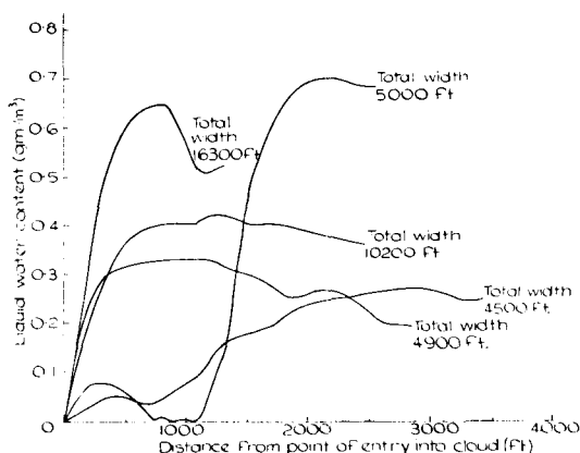
Fig. 5. Variation of water content with distance.
