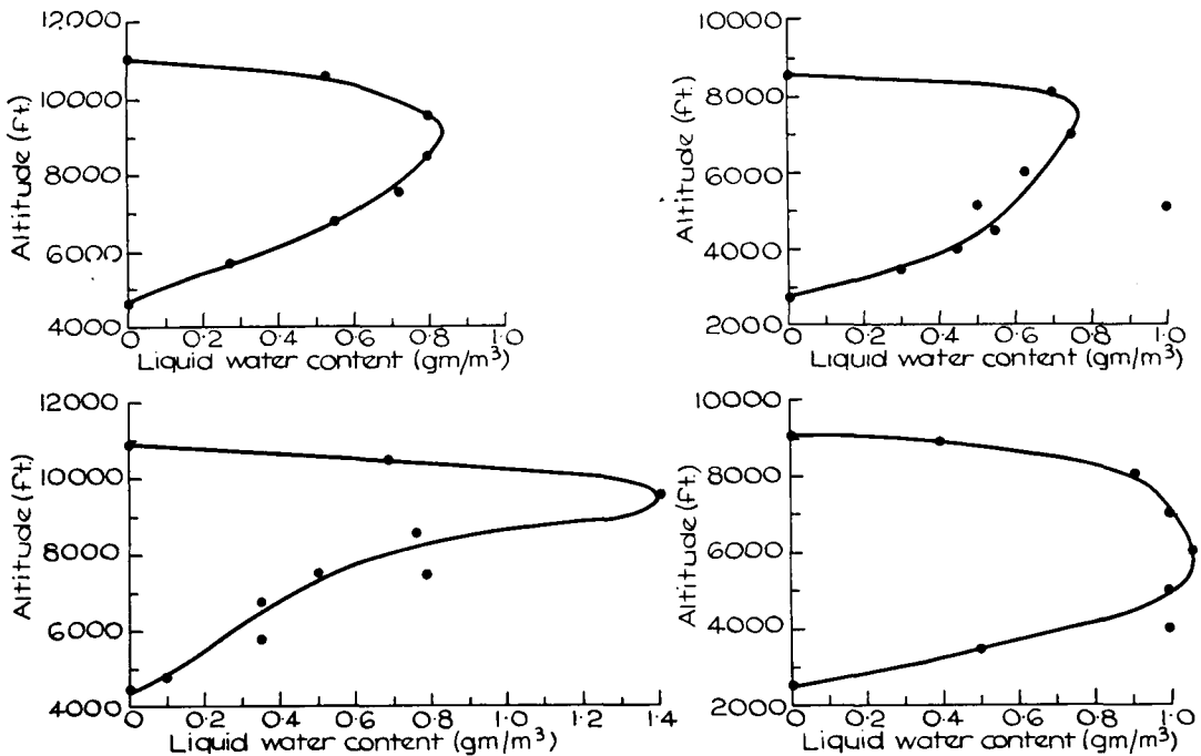
Fig. 6. Variation of peak water content with height.
