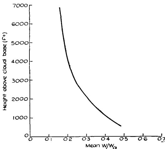
Fig. 8. Mean ratio W/W_a versus height above base.
