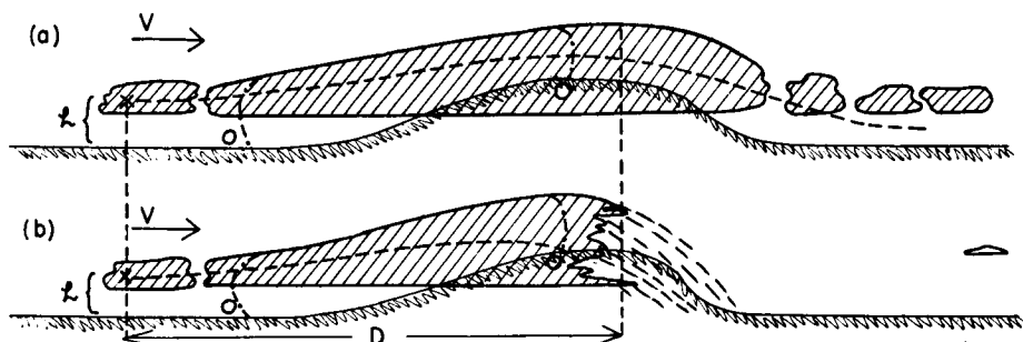
Fig. 1. Formation of snow in mountain clouds. An ice crystal introduced at a height h (several hundred m above ground) into clouds windward of the mountain has a trajectory shown by the pecked lines (partly lying within the region of orographic updraught). The crystal is initially a distance D from the region where air begins to descend in the lee of the mountain. In (a), (D/V) , where V is the mean wind speed, is considerably less than 1,500 sec; the crystal attains a radius of less than about 200 \mu , settles relative to the air less than 200 m, and evaporates in the lee of the mountain. In (b), (D/V) is rather more than 1,500 sec; the crystal attains a diameter of about 1 mm, settles relative to the air several hundred m, and thus is precipitated upon the mountain. If an appropriate concentration of crystals is introduced, each follows a similar trajectory, and the vapour condensed in the cloud is consumed in producing the snowfall, so that the mountain cloud disappears where the air begins to descend behind the mountain.
