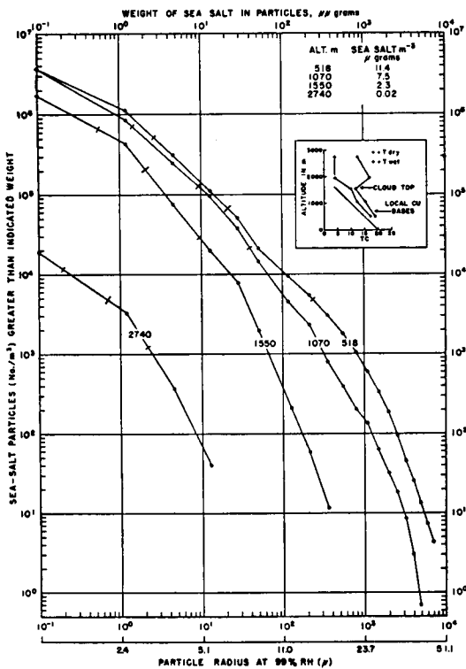
Fig. 8. An example of the decrease, with altitude, in the numbers of salt particles in Hawaii. Approximate position 21^{\circ} 30' N , 157^{\circ} 40' W ; Time 1300 LCT, 30 May 1952. Surface wind 80 deg. force 4 to 5. Note that the region of cloud development is one of rapid decrease with height in the numbers of the larger nuclei. (The lines are drawn between the observed values as an aid to the eye in following the trends of the various observed distributions.)
