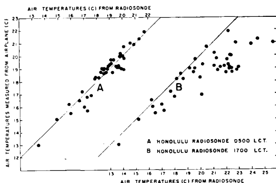
Fig. 2. Comparison of air temperatures observed from the salt-nuclei-sampling aircraft near cloud-base altitudes (see sampling area on fig. 1), with Honolulu radiosonde temperatures on the same day and at comparable altitudes.
