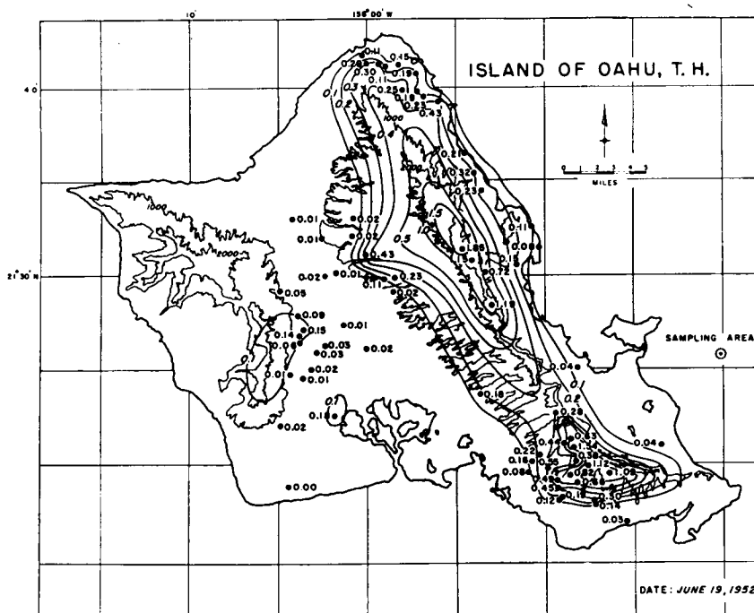
Fig. 1. Example of isohyetal maps used in deriving the total rain amounts shown on table 1, column 2. Rainfall amounts shown here are given in inches.
