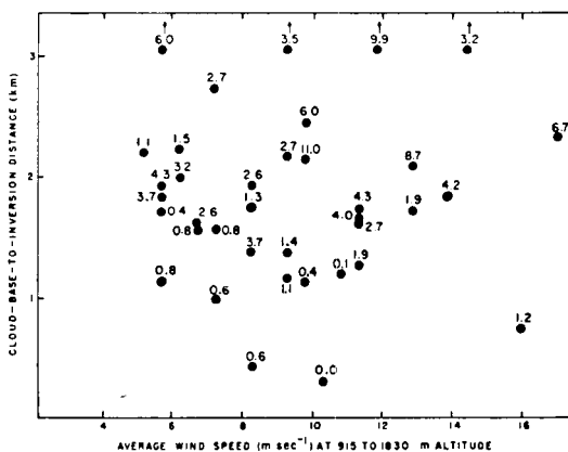
Fig. 6. Repetition of Figure 4, substituting wind speed at cloud levels for numbers of salt particles.
