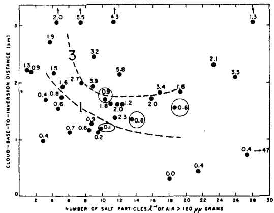
Fig. 7. The quotient of the total daily rain amounts and a function of wind speed, related to the number of salt nuclei in the air and to the cloud-base-to-inversion distances. See text for further discussion.
