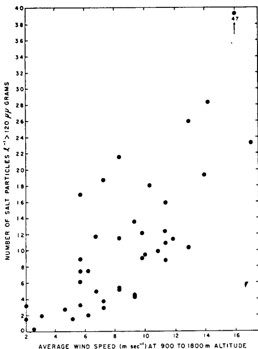
Fig. 5. Number of salt particles near cloud-base altitudes, related to the average wind speed at altitudes between 900 and 1800 meters. (See WOODCOCK, 1953, for more detailed indication of dependence of salt nuclei upon wind).
