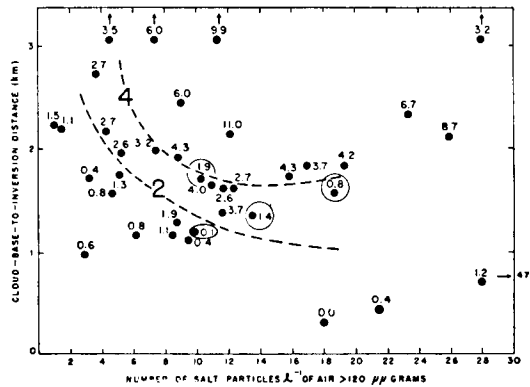
Fig. 4. Total daily amounts of rainfall on Oahu, expressed in units of 10^2 metric tons, related to the numbers of salt nuclei in the air and to the cloud-base-to-inversion distances. See text for further discussion.
