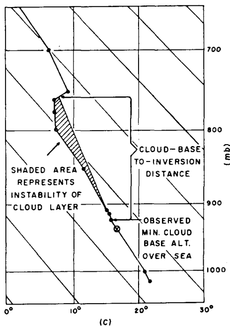
Fig. 3. Pseudo-adiabatic chart of Honolulu radiosonde record (1500Z, 26 February 1952) illustrating derivation of the cloud-base-to-inversion distances and the instability areas shown on table 1, columns 5 and 13. The circled X marks a temperature and pressure observed on the same day from aircraft over the windward sea.
