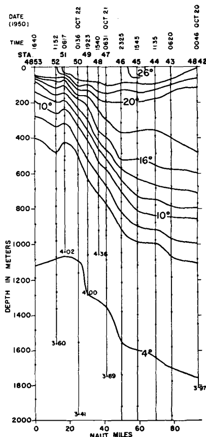
Fig. 3. Section 1: Temperature.
