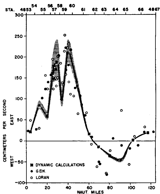
Fig. 7. Surface velocity—section 2.
