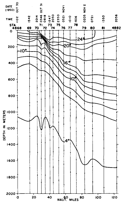
Fig. 5. Section 3: Temperature.
