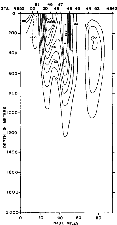
Fig. 9. Section 1—velocity cm/sec.
