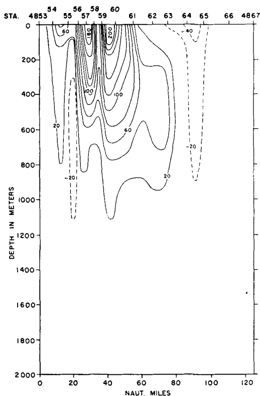
Fig. 10. Section 2—velocity cm/sec.
