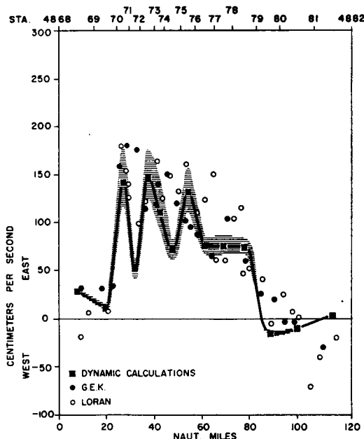
Fig. 8. Surface velocity — section 3.
