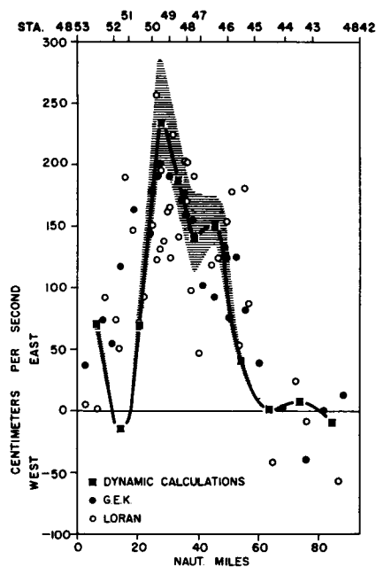
Fig. 6. Surface velocity—section 1.
