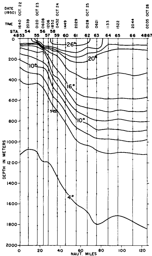
Fig. 4. Section 2: Temperature.
