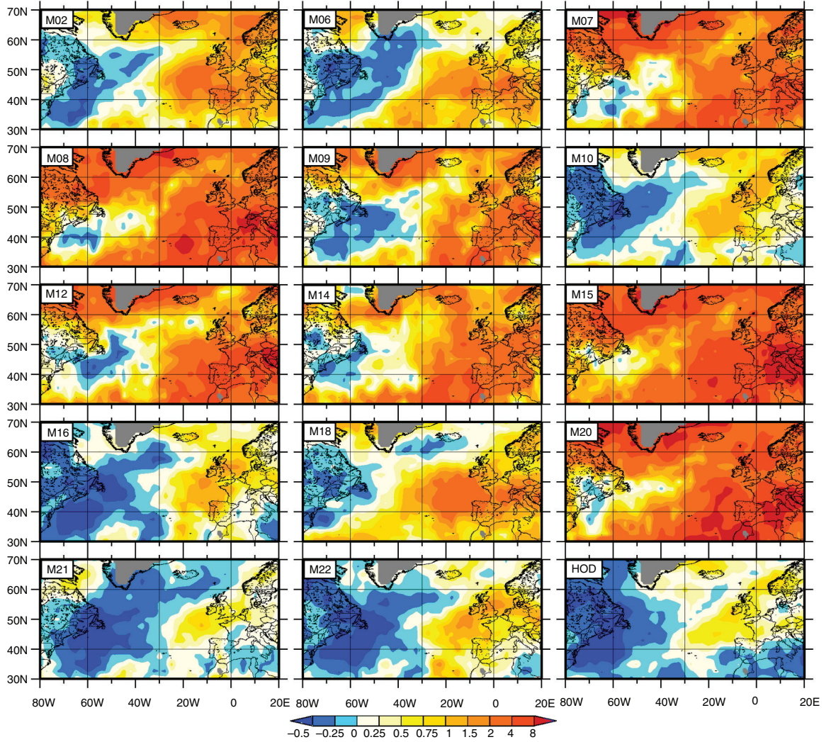
Fig. 6. Estimated dispersion statistic \phi' quantified with 4 \cdot (s_{\bar{\phi}})^2 - 1 for each of the 15 methods (M02–M22, HOD) derived from ERA-Interim (1979–2010). Derived from ERA-Interim (1979–2010).
