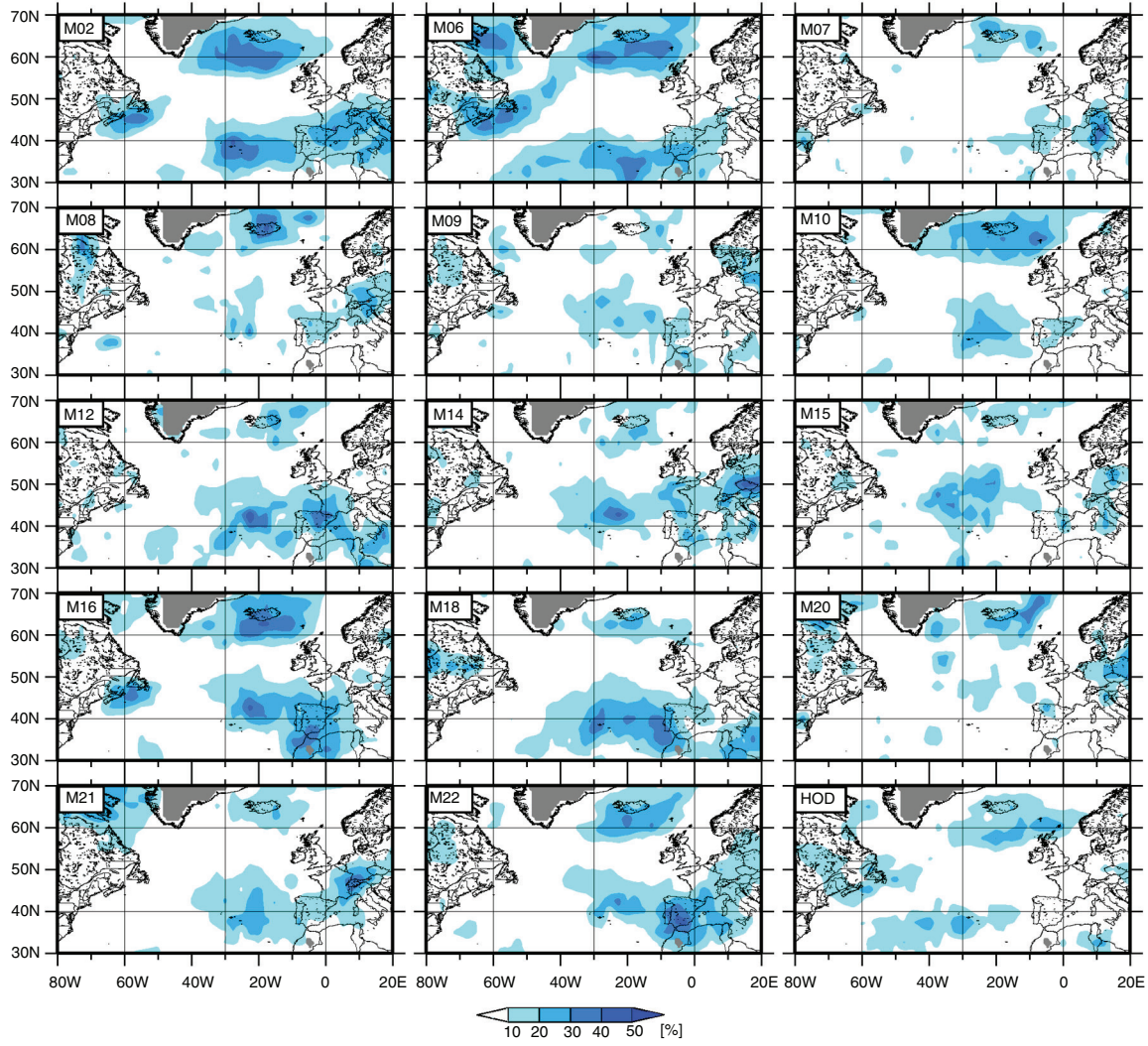
Fig. 9. Relative effect of North Atlantic Oscillation (NAO) on dispersion following \beta^2(s_x)^2/(s_{\sqrt{y}})^2 for each of the 15 methods (M02–M22, HOD) derived from ERA-Interim (1979–2010).
