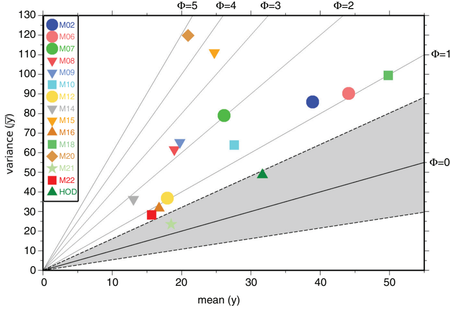
Fig. 5. Variance (s_y)^2 (y-axis) and mean of cyclone track counts per winter \bar{y} (x-axis) for the grid point 55^\circ\text{N} , 5^\circ\text{W} for each method (M02–M22, HOD). Isolines of dispersion statistic \phi are depicted in black (for values 0–5). The grey area depicts a 95% (bootstrap) confidence interval for the variance, under the assumption of no overdispersion.
