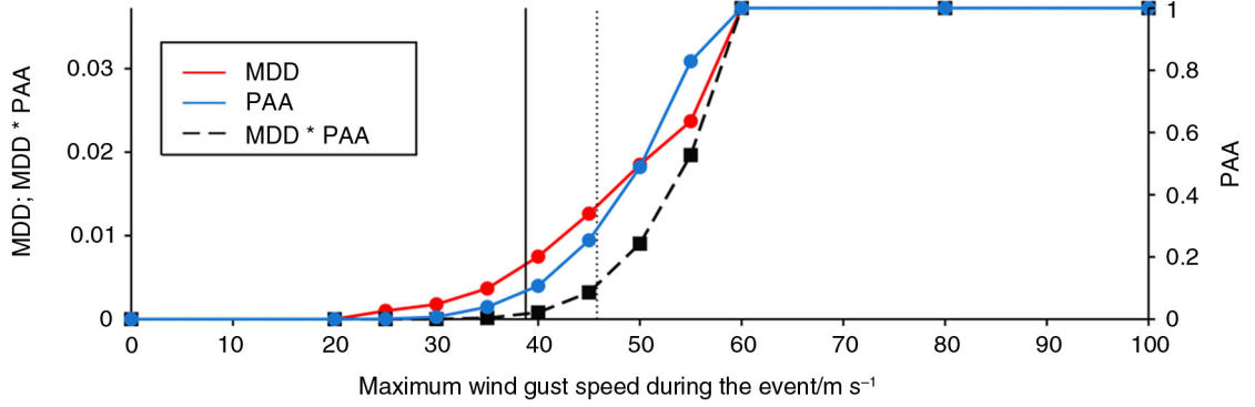
Fig. 3. Mean damage degree (red; left y-axis), percentage of assets affected (blue; right y-axis), and product of MDD and PAA (black; left y-axis) as a function of maximum wind gust speed during the windstorm event. A linear interpolation was applied between two consecutive points (denoted with a straight line segment). The maximum downscaled surface wind gust speed over Switzerland during ‘Lothar’ (added with 7 \text{ m s}^{-1} ; i.e. the average bias of estimated surface wind gust speeds using the WPD method compared to instrumental wind gust speed measurements in case of ‘Lothar’; see Table 1) is marked by the solid (dotted) vertical line.
