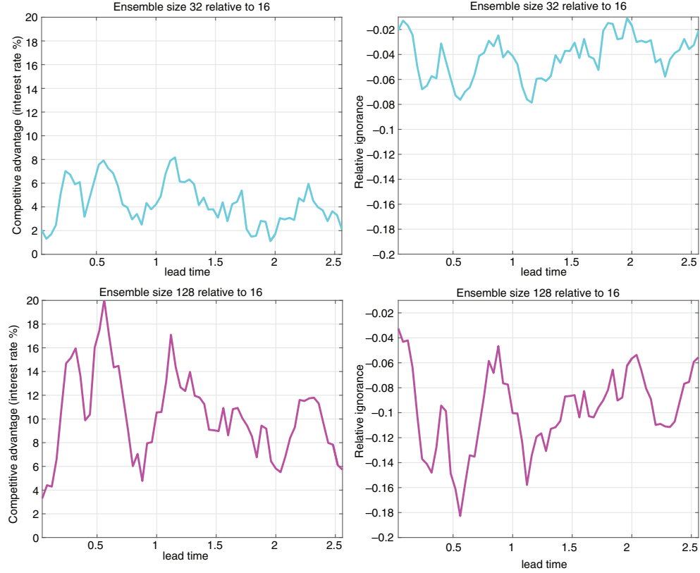
Fig. 4. Moore-Spiegel system with inverse noise. The two graphs on the left show the competitive advantage as a function of lead-time for an ensemble size of 32 relative to 16 as functions of lead-time (top) and 128 relative to 16 (bottom). Each curve corresponds to a slice through Fig. 3. The IGN scores for the same comparisons are shown on the right. Note the symmetry between ignorance and competitive advantage [flipping over ( y \rightarrow -y ) in a graph in the right column leads yields the pattern of a curve on the left].
