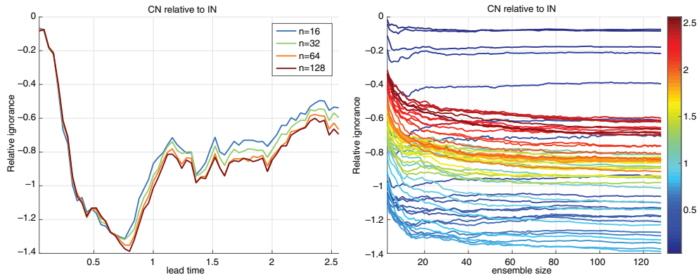
Fig. 8. Contrasting skill due to data assimilation scheme: Moore–Spiegel system. The skill of competing forecast systems which differ only in the data assimilation scheme is contrasted in the Moore–Spiegel system: each panel shows IGN of CN-based forecasts relative to those of IN-based forecasts, thus negative values imply more skill in the CN method. Note that all values are negative. Left: Ignorance as a function of lead time for four ensemble sizes (16, 32, 64 and 128). Note that the forecast system using CN gains additional skill above the one using IN as the ensemble size increases. Right: Ignorance as a function of ensemble size for a variety of lead times (as indicated by the colour bar on the right-hand side of the panel). Note that the benefit of using CN is greatest in the medium range, lead times between 0.5 and 0.9; while the advantage continues to exceed half a bit (a 40 % gain in probability, on average) at longer lead times, it is less than a tenth of a bit at short lead times. This suggests that the CN data assimilation might require improvement (to justify its added cost) if the focus is on shorter lead times. Also note in the right panel that for longer lead times (reddish) the skill curves are still sloping down even at the largest ensembles tested, indicating that the CN-based forecasts are improving faster as the ensemble size is increased even at the largest ensembles tested.
