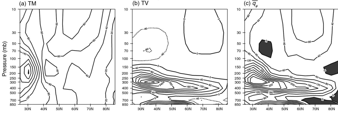
Fig. 10. (a) TM, (b) TV and (c) \overline{q_M} based on the DJF-mean zonal mean basic state in the NH extratropics. For the definitions and formulas of TM, TV and \overline{q_M} , see details in the text, and all of them are scaled by a^2/10 in the plots. In (c), regions with negative values are shaded.
