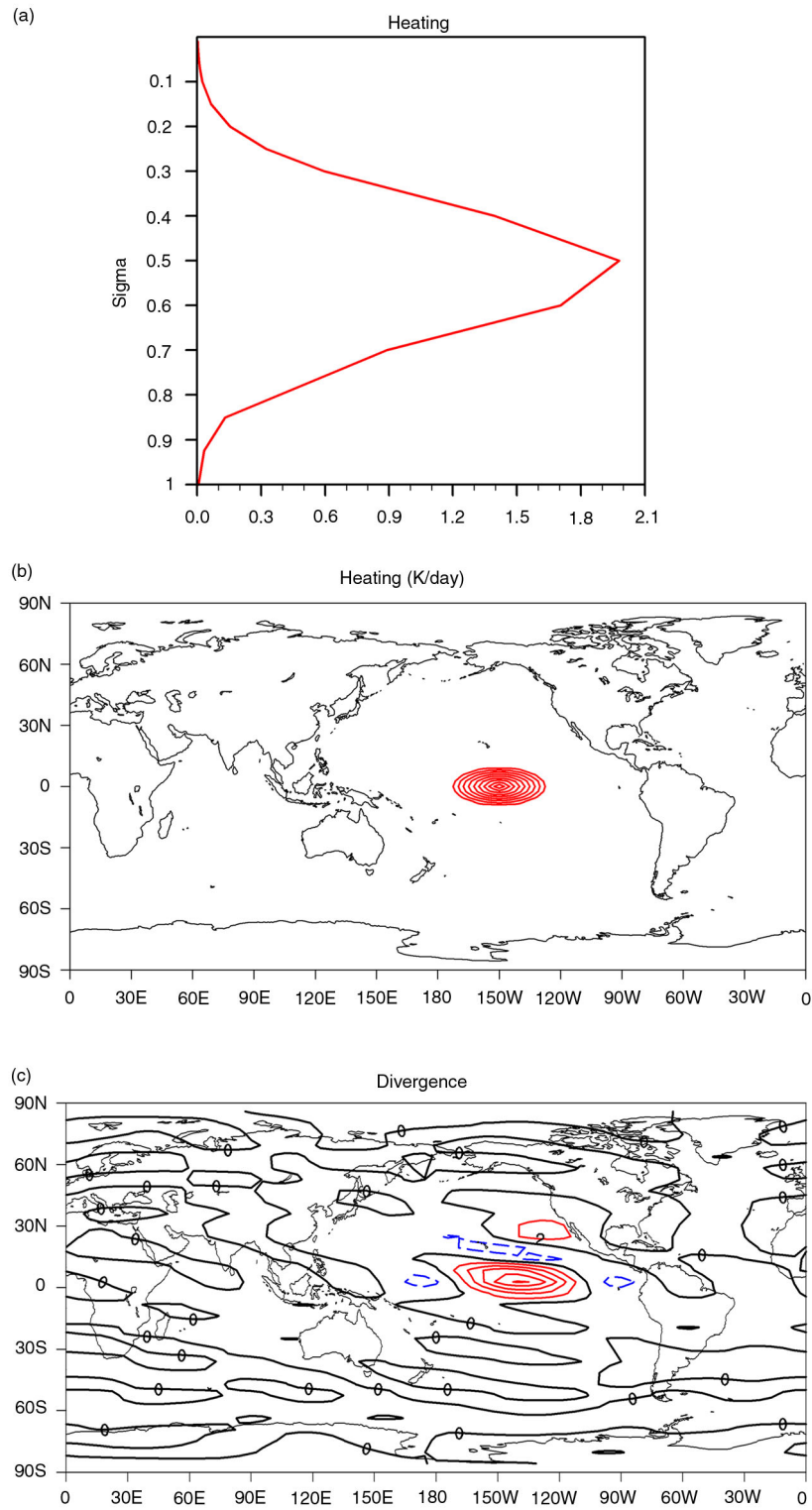
Fig. 11. (a) Vertical and (b) horizontal distributions of the tropical heating used in Exp1. Contour interval in (b) is 0.1^{\circ} \text{ K d}^{-1} . (c) Divergence at 200 hPa (in 10^{-7} \text{ s}^{-1} ) computed from the steady LBM response to the tropical heating in (a) and (b).
