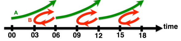
Fig. 3. Implementation of the LETKF-RIP scheme in the WRF model. Loop A is the zero iteration performing regular LETKF with a 6-hour ensemble forecast. Loop B includes the use of the no-cost smoother and forecast-analysis steps with a cycle shorter than Loop A. Adopted from Kalnay and Yang (2010).
