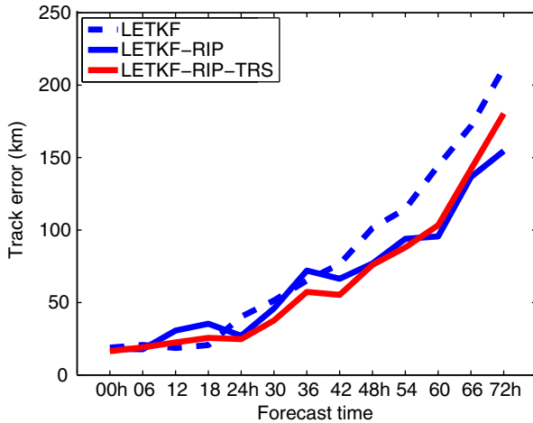
Fig. 18. Mean cross track error from the LETKF and LETKF-RIP forecasts at different forecast hours averaged from the cases initialised at 0000 UTC 9 September to 0600 UTC 12 September with a 6-hour interval.
