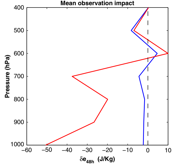
Fig. 13. Vertical distribution of the observation impact per dropsonde. The red line denotes the results obtained with the LETKF-RIP experiment and the blue line denotes the LETKF results.
