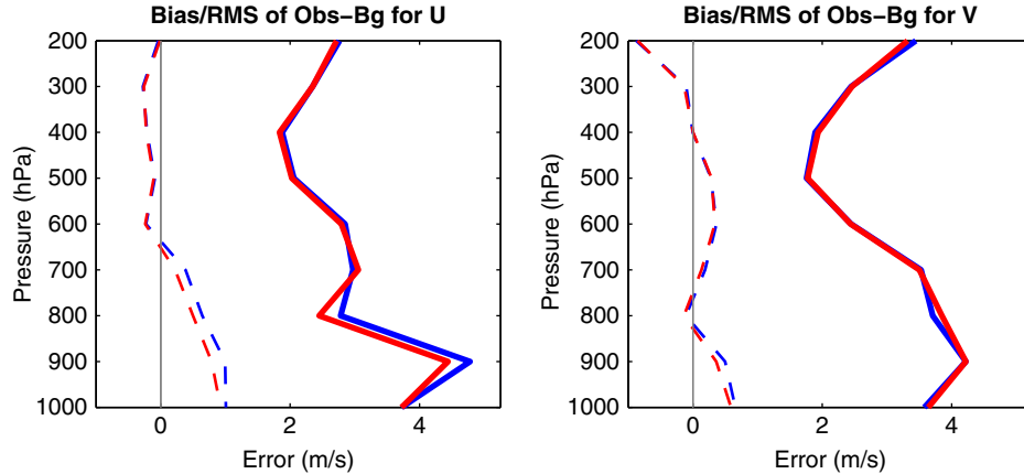
Fig. 6. (a) Bias (dashed lines) and RMS (solid lines) of the innovation vectors for the zonal velocity, (b) the same as (a) except with meridional velocity. Results with the LETKF and LETKF-RIP background are denoted in blue and red colours, respectively.
