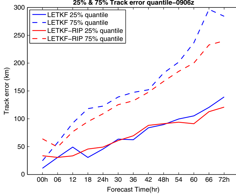
Fig. 11. The 25% and 75% quantiles of the ensemble track errors from the LETKF and LETKF-RIP ensemble forecasts initialised at 0600 UTC 9 September.
