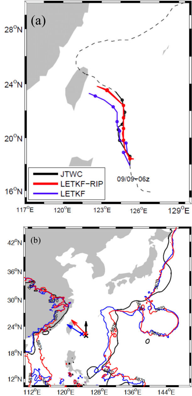
Fig. 9. (a) Typhoon track prediction initialised at 0600 UTC 9 September with the LETKF (blue) and LETKF-RIP analysis (red line). (b) The 5880 isolines of the 500 hPa geopotential height at 1200 UTC 11 September with the same initial conditions as used in (a). The arrows indicate the typhoon moving direction at 1200 UTC 11 September from the forecasts and observation (in black).
