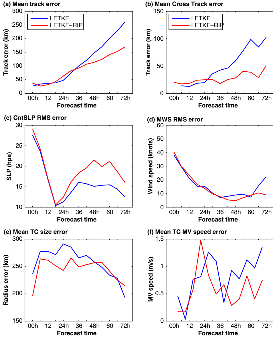
Fig. 8. Mean errors associated with typhoon parameters from the LETKF and LETKF-RIP forecasts at different forecast hours: (a) absolute track; (b) cross track error; (c) sea-level pressure at typhoon centre; (d) maximum wind speed; (e) size of the typhoon; and (f) the mean translation speed of the typhoon
