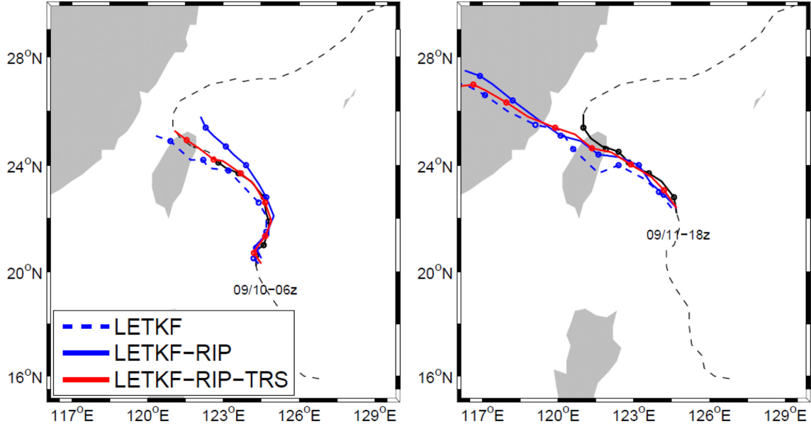
Fig. 16. (a) Typhoon track prediction initialised at 0600 UTC 10 September with the LETKF (blue dashed line), LETKF-RIP analysis (blue solid line) and LETKF-RIP-TRS analysis (red solid line). (b) Same as (a) except the initial time is 1800 UTC 11 September.
