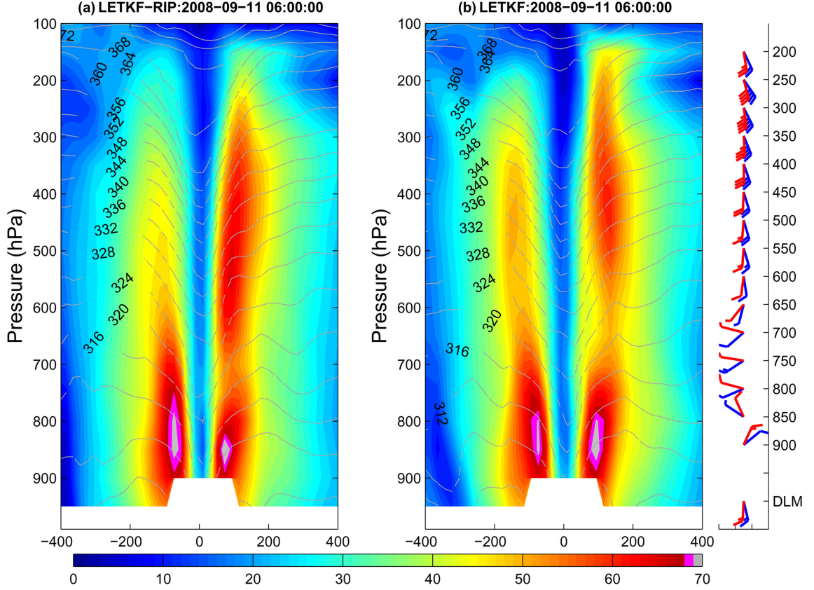
Fig. 10. East-west cross section of the typhoon vertical structure from the 2-day forecasts initialised by: (a) the LETKF-RIP and (b) the LETKF analyses at 0600 UTC 9 September 2008. The colour shading denotes the wind speed and the contours denote the potential temperature. The blue (red) wind bars on the right-hand side denote the steering flow for the typhoon in the LETKF (LETKF-RIP) forecast in the vertical, and those at the bottom are the deep layer mean wind.
