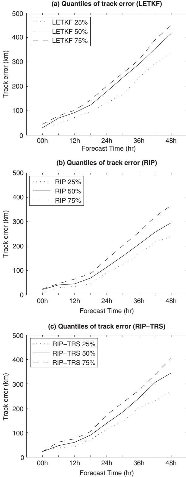
Fig. 17. The 25%, 50% and 75% quantiles of the ensemble track errors from: (a) the LETKF, (b) LETKF-RIP and (c) LETKF-RIP-TRS ensemble forecasts initialised at 1800 UTC 11 September.
