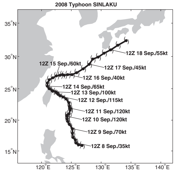
Fig. 1. JTWC best track and intensity of typhoon Sinlaku 2008. Data are plotted every 6-hour.
