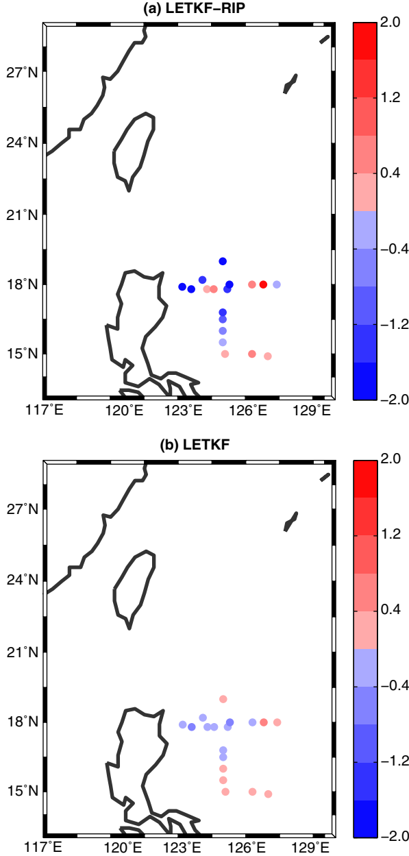
Fig. 12. Forecast sensitivity verified at 0600 UTC 11 September with respect to the dropsondes at 0600 UTC 9 September with results of the (a) LETKF-RIP and (b) LETKF analyses and forecasts. The unit of the colour bar is \text{JKg}^{-1} .
