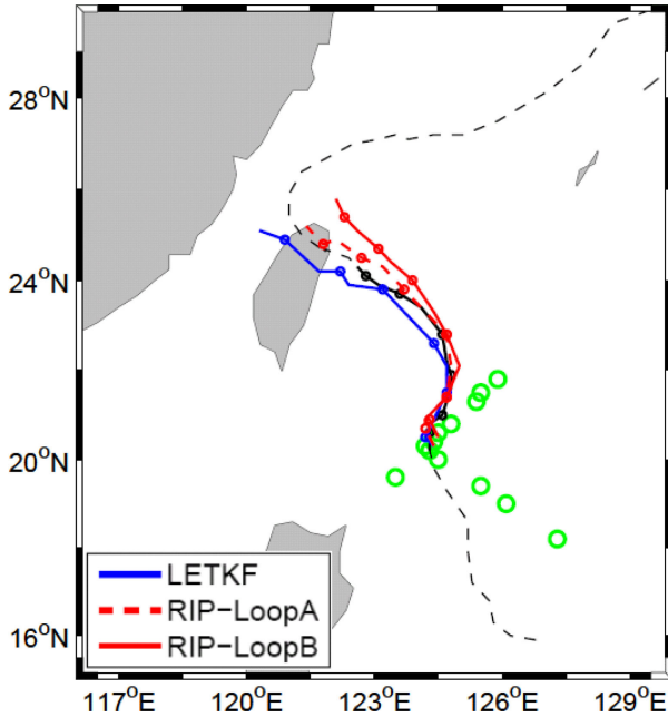
Fig. 14. Typhoon track prediction initialised at 0600 UTC 10 September with the LETKF (blue) and LETKF-RIP analysis from Loop A (red dashed line, also the first iteration) and from Loop B (red solid line, also the second iteration). Green dots are the locations of the dropsondes.
