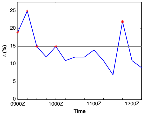
Fig. 15. Time series of the ratio \varepsilon . The grey line indicates the stopping criterion (15%) to automatically switch the RIP iterations on ( \varepsilon \geq 15\% ) or off.
