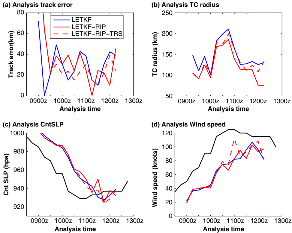
Fig. 7. Analysis errors of typhoon-related parameters: (a) track, (b) 30-kts wind radii, (c) sea-level pressure at typhoon centre and (d) maximum surface wind.
