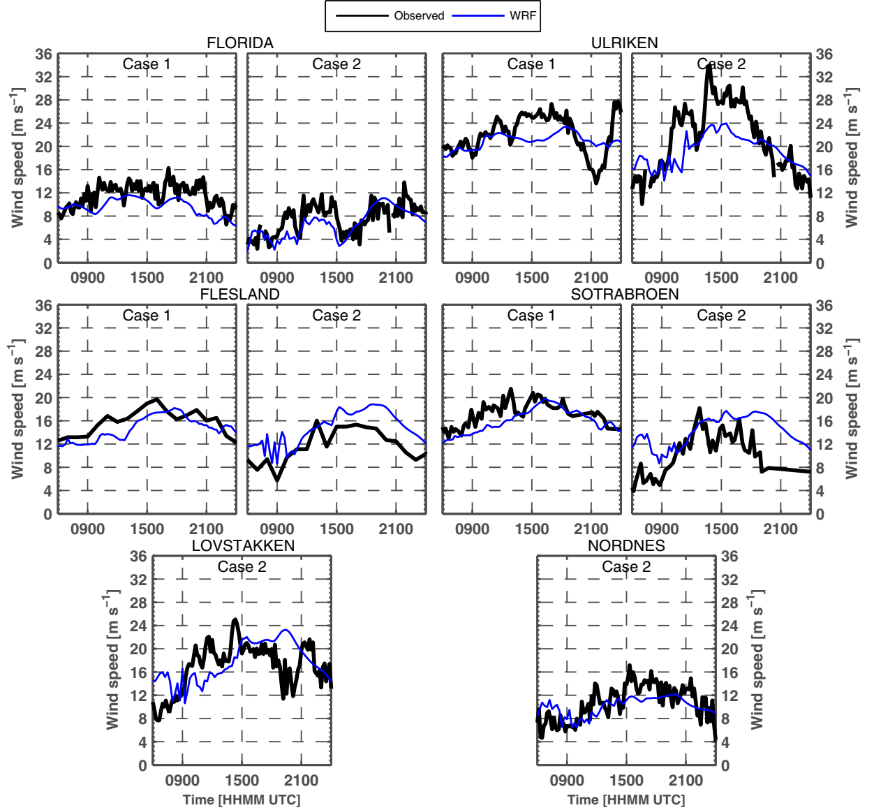
Fig. 8. Observed and simulated wind speed at selected AWSs on 10 January 2009 (Case 1) and 25 December 2011 (Case 2). The simulation results are from the innermost domain (500-m horizontal resolution).
