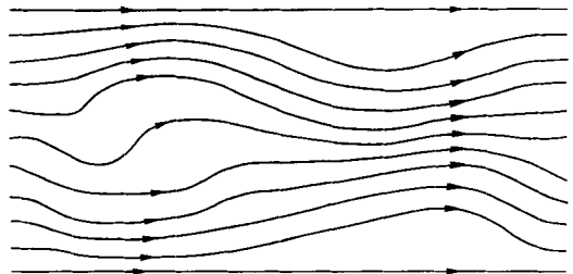
Fig. 4. Streamlines at some distance downstream of an obstacle whose area in the plane of the motion, Q = H^2/10 \pi . The internal Froude number, F^2 = 1/5 \pi^2 .
