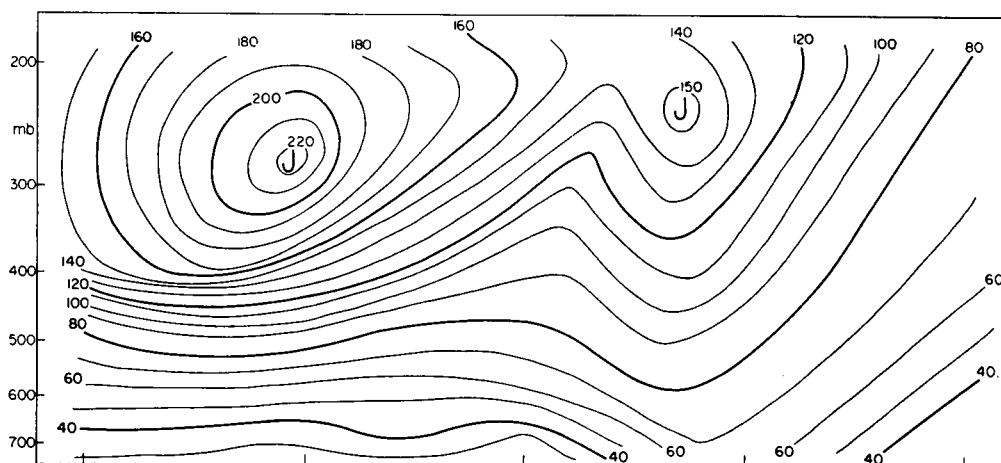
Fig. 10 c. Cross-section of isotachs, November 13, 1951, 1500 GMT. Marks at bottom correspond to tick marks of fig. 5 c. For details of construction of figure see text. "J" denotes jet stream center.
