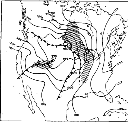
Fig. 1a. Surface isobars (mb) and fronts, November 12, 1951, 1830 GMT. Area of steady precipitation is shaded.
