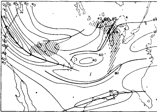
Fig. 5 a. Isotachs at 500 mb (knots), November 12, 1951, 1500 GMT. Heavy lines mark jet stream axes. Tick marks along axis of principal current serve to identify the horizontal axis of fig. 10 a. Precipitation areas are shaded. Dashed lines give 3-hour surface isallobars (mb).
