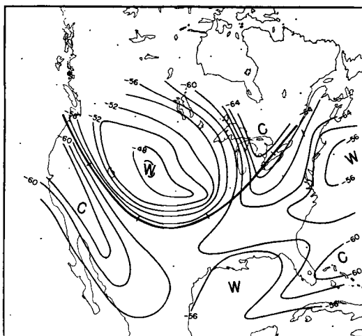
Fig. 8. Isotherms ( ^{\circ}\text{C}. ) at 200 mb, November 13, 1951, 1500 GMT. Jet stream center at 300 mb marked by heavy line. Tick marks along jet axis serve to identify the horizontal axis of fig. 9.
