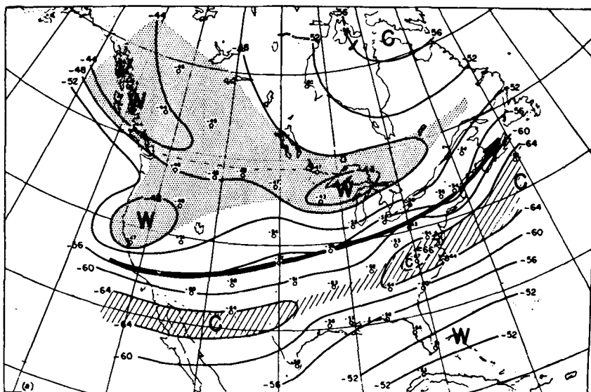
Fig. 7. "Isotherms ( ^{\circ} C.) at 200 mb, January 28, 1947, 0300 GMT. Jet stream center at 300 mb marked by heavy line." (From RIEHL, 1948.)
