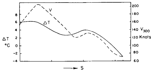
Fig. 9. Wind speed at 300 mb (knots), and temperature gradient ( ^{\circ}\text{C}. ) at 200 mb taken over distance of 250 km normal to jet axis (heavy line) of fig. 8. Marks at bottom correspond to tick marks along jet axis of fig. 8.
