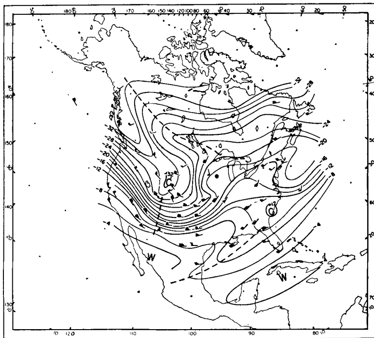
Fig. 2c. Winds and isotherms at 500 mb, November 13, 1951, 1500 GMT. Axes of minimum and maximum temperature gradient are marked by dashed lines. "W" denotes warm center and "C" denotes cold center. On wind vectors a long barb denotes 10 knots, a short barb 5 knots, and a heavy triangular barb 50 knots. Heavy dot marks position of surface low pressure center.
