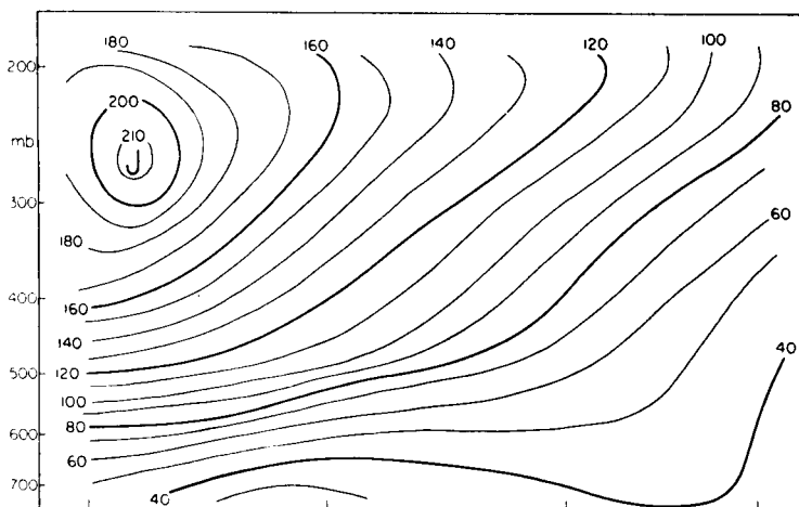
Fig. 10 a. Cross-section of isotachs (knots) along axis following jet stream core, November 12, 1951, 1500 GMT. Marks at bottom correspond to tick marks of fig. 5 a. For details of construction of figure see text. "J" denotes jet stream center.
