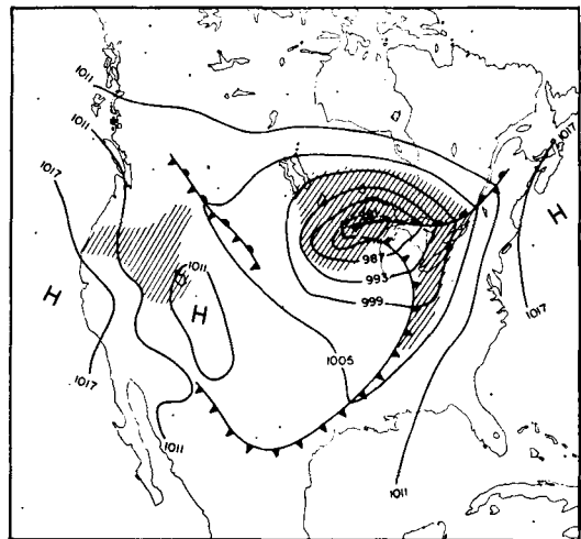
Fig. 1d. Surface isobars and fronts, November 14, 1951, 0630 GMT.
