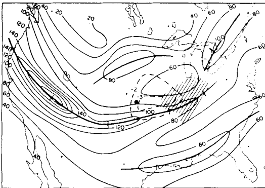
Fig. 5 b. Isotachs at 300 mb, November 13, 1951, 0300 GMT. Heavy lines mark jet stream axes. Tick marks correspond to those along horizontal axis of fig. 10 b. Heavy dot marks position of surface low pressure center.
