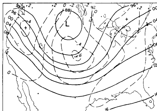
Fig. 4 c. Contours of the 300-mb surface and 12-hour height changes, November 13, 1951, 1500 GMT.
