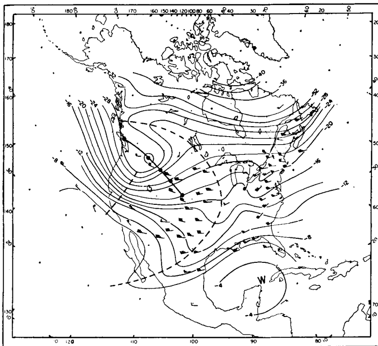
Fig. 2a. Winds and isotherms ( ^{\circ}\text{C}. ) at 500 mb, November 12, 1951, 1500 GMT. Progression of cold dome in 12-hourly steps, November 12, 0300 GMT to November 14, 0300 GMT, is marked by heavy line. Axes of minimum and maximum temperature gradient are marked by dashed lines. "W" denotes warm center and "C" denotes cold center. On wind vectors a long barb denotes 10 knots, a short barb 5 knots, and a heavy triangular barb 50 knots.
