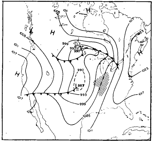
Fig. 1b. Surface isobars and fronts, November 13, 1951, 0630 GMT.
