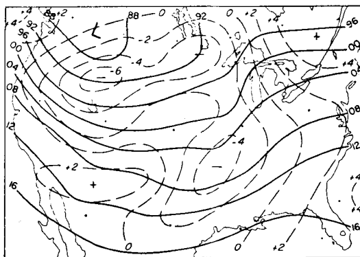
Fig. 4 a. Contours of the 300-mb surface (100's feet, first digit omitted) and 12-hour height changes (100's feet), November 12, 1951, 1500 GMT.
