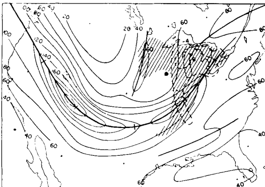
Fig. 5 c. Isotachs at 300 mb, November 13, 1951, 1500 GMT. Heavy lines mark jet stream axes. Tick marks correspond to those along the horizontal axis of fig. 10 c. Heavy dot marks position of surface low pressure center.
