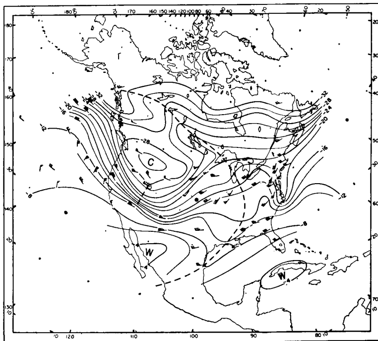
Fig. 2b. Winds and isotherms at 500 mb, November 13, 1951, 0300 GMT. Axes of minimum and maximum temperature gradient are marked by dashed lines. "W" denotes warm center and "C" denotes cold center. On wind vectors a long barb denotes 10 knots, a short barb 5 knots, and a heavy triangular barb 50 knots. Heavy dot marks position of surface low pressure center.
