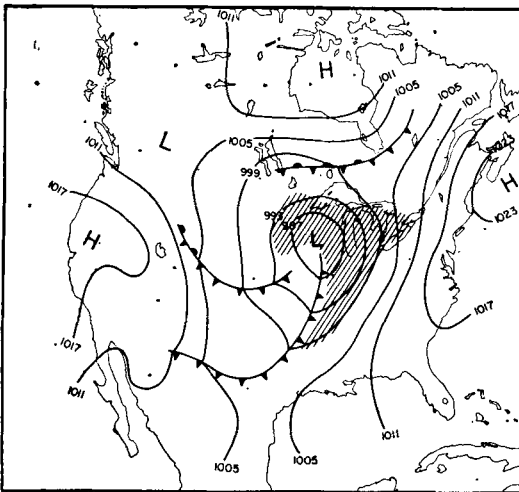
Fig. 1c. Surface isobars and fronts, November 13, 1951, 1830 GMT.
