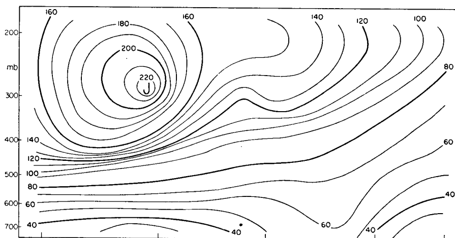
Fig. 10 b. Cross-section of isotachs, November 13, 1951, 0300 GMT. Marks at bottom correspond to tick marks of fig. 5 b. For details of construction of figure see text. "J" denotes jet stream center.
