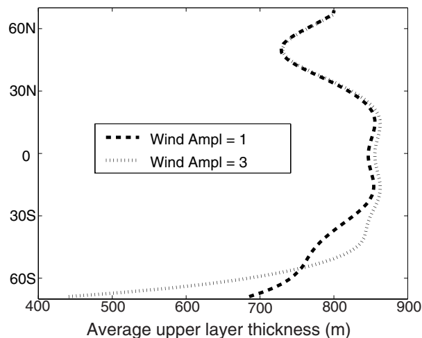
Fig 16. Zonally averaged upper layer thickness for experiments 3 (wind amplification factor of 1) and 6 (wind amplification factor of 3). The response to stronger winds occurs mainly in the Southern Hemisphere. In the case of stronger SO winds, the upper layer in the south becomes thin so that the ocean takes up heat from the atmosphere. For standard winds, the upper layer in the south is thicker (warmer) than the atmospheric thickness and, therefore, it loses heat to the atmosphere. In this case buoyancy is provided by the freshwater flux (see Fig. 11).
