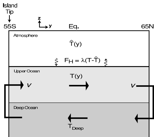
Fig 8. Slab model of the ocean and atmosphere from 55^\circ\text{S} to 65^\circ\text{N} . The upper layer presents the atmosphere which has a fixed y -dependent temperature profile, \hat{T}(y) , depicted in Fig. 9. Below the atmosphere lies the upper ocean which exchanges heat with the atmosphere in an amount proportional to (T - \hat{T}(y)) . A constant flow of water flows northward in this layer at a constant velocity, v , determined by the Belt Constraint (3) and the zonal wind stress at 55^\circ\text{S} . North of 65^\circ\text{N} the water is subducted to the deep layer, returns south, and is upwelled again south of 55^\circ\text{S} .
