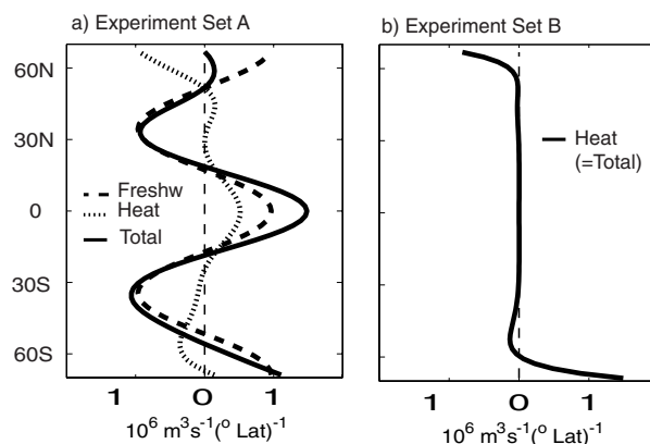
Fig. 11. Buoyancy forcing for sets A and B. An imposed buoyancy flux at the surface is converted to a source or sink of upper layer water. For set A, the freshwater flux (dashed line) is a fixed profile, while the heat flux (dotted line) depends on the upper layer thickness (see text for more details). The buoyancy south of 55°S is provided by the freshwater flux which allows a negative heat buoyancy flux. For set B, the freshwater flux is neglected and the heat fluxes at the poles are exaggerated compared to the equator. In the absence of freshwater flux, which provides buoyancy to the SO, the heat flux itself must provide the required buoyancy. Both heat flux profiles are for a wind amplification factor of 1 (experiments 3 and 9). Note that, for stronger winds, the heat buoyancy flux in the SO is positive also for the experiments in set A because the freshwater flux is then inadequate for providing the required buoyancy.
