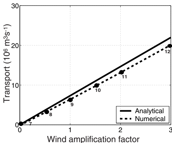
Fig 15. Transport across 55^\circ\text{S} for experiments in set B. As in Fig. 13, the solid line is the analytical transport determined by the Belt Constraint (3), while the dashed line shows the dependence of the numerical transport on the increased winds. Each bullet is labeled by its experiment number (Table 1). Here, too, the numerical flow agrees very closely with the Belt Constraint.
