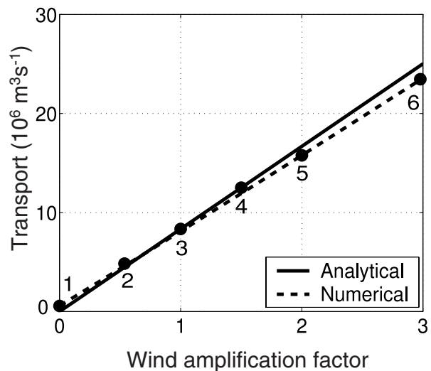
Fig 13. Transport across 55°S, the latitude just south of the island (Fig. 9) for experiments in set A. The solid line is the analytical transport determined by the Belt Constraint (3). The dashed line shows the dependence of the numerical transport on the increased winds. Each bullet indicates a different run and is labeled by its experiment number (Table 1). The numerical flow agrees very closely with the Belt Constraint. The minute differences are due to lateral friction, linear drag and advection in the numerical model as indicated in Fig. 14.
