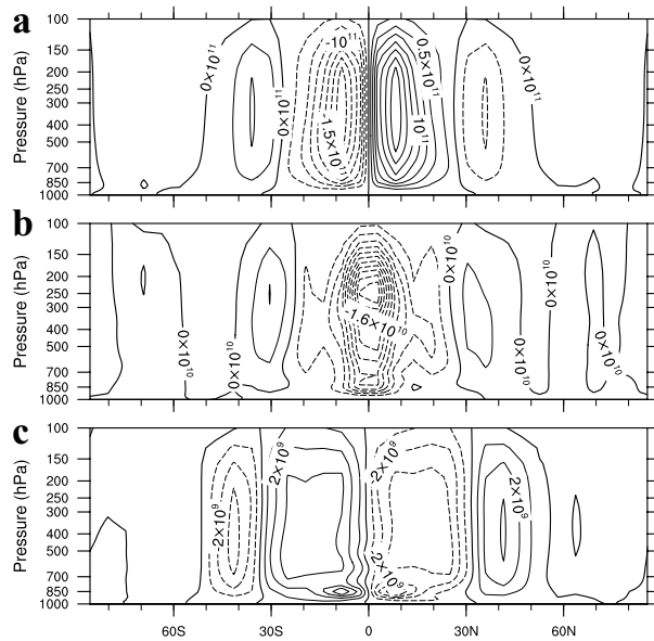
Fig. 3. Zonal mean meridional streamfunction ( \text{kg s}^{-1} ): (a) streamfunction in reference climate; (b) change when going to first-order perturbation; (c) change when going to second-order perturbation. All plots for CCM3 model.
