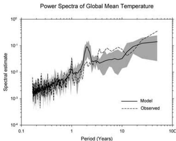
Fig. 3. Power spectra of the global mean T2m from the ECHO-G CTL (solid line) and HadCRUT2 observations (dashed line, 1901–2000). The shading indicates the maximum and minimum spectral estimates from 10 100-yr sections of the ECHO-G CTL, and the solid line is an average of the 10 power spectra.
