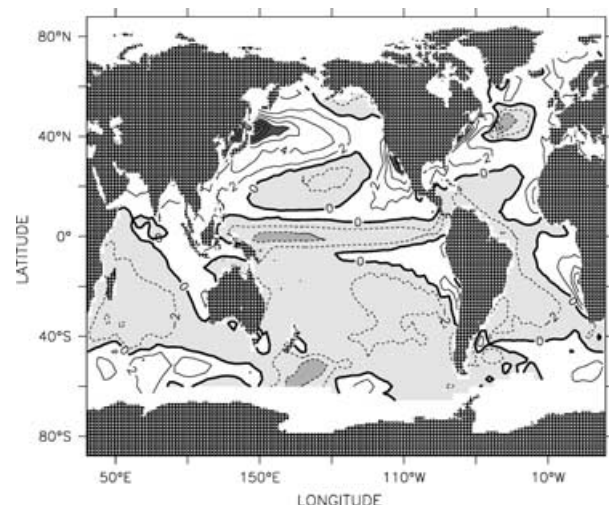
Fig 2. Mean model SST bias (modelled minus observed). Observed SST are from Reynolds and Smith (1994). Mean model SST is calculated from years 31 to 400 of the control run. The contour interval is 2°C. Negative values are shaded lightly, and positive values greater than 8°C are shaded the darkest.
