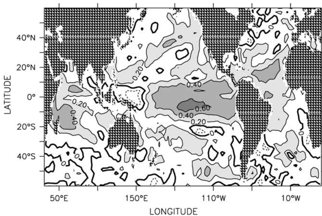
(a) Correlation
