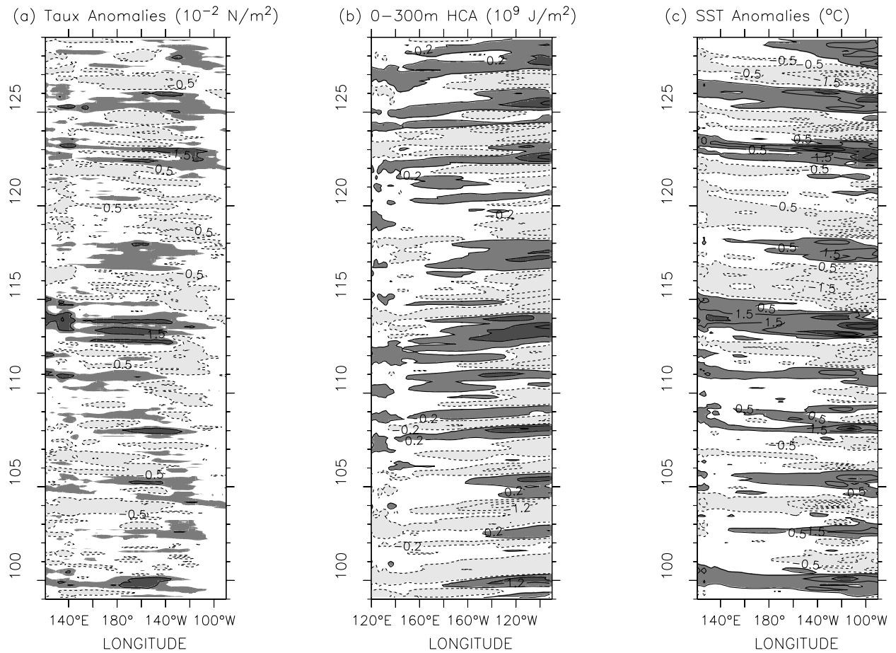
Fig 6. Hovmoeller diagrams of 2^{\circ}\text{S} – 2^{\circ}\text{N} averaged anomalies of (a) zonal wind stress, (b) 0–300 m heat content and (c) SST. A three-month running mean has been applied. The contour intervals for (a), (b) and (c) are 2, 1 and 1, respectively.
