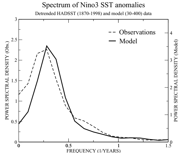
Fig. 4. Modelled and observed Niño3 SSTa power spectra. Modelled spectra calculated from years 31 to 400 of the control run. Observations (1870–1998) are the HADISST data set (Rayner et al., 2003) from the Hadley Centre, UK Meteorological Office. Data are detrended, and spectra are calculated using a Bartlett window of 8 yr.
