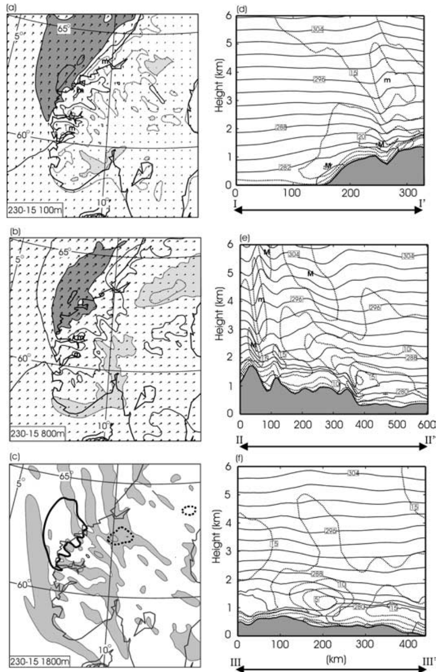
Fig 3. Horizontal wind maps for three levels (left column, isotachs every 4 \text{ m s}^{-1} ) and cross-sections, shown in Fig. 2a, I, II and III (right column) of potential temperature (contours every 2 K) and wind speed (isotachs every 2.5 \text{ m s}^{-1} ) for large-scale wind direction 230^\circ and speed 15 \text{ m s}^{-1} . Upper left panel: surface (approximately 100 m above ground). Isotachs: solid contours, 12 \text{ m s}^{-1} and more; stippled contours, less than 12 \text{ m s}^{-1} . Maximum areas more than 16 \text{ m s}^{-1} and minimum areas less than 4 \text{ m s}^{-1} are shaded grey. Other minima are marked with an "m". Middle left panel: aloft (approximately 700 m above ground). Isotachs as before, but solid contours are 14 \text{ m s}^{-1} and more and stippled contours less than 14 \text{ m s}^{-1} . Maximum areas more than 22 \text{ m s}^{-1} and minimum areas less than 10 \text{ m s}^{-1} are shaded grey (maximum area darker than minimum area). Lower left panel: approximately 1800 m above ground. Isotachs as above, but the contour for 14 \text{ m s}^{-1} is omitted: heavy solid contours, 18 \text{ m s}^{-1} or more; heavy stippled contours, wind speed of 10 \text{ m s}^{-1} and less; shaded areas, two stippled contours of negative omega (positive vertical wind component), -0.001 \text{ hPa s}^{-1} and -0.01 \text{ hPa s}^{-1} .
