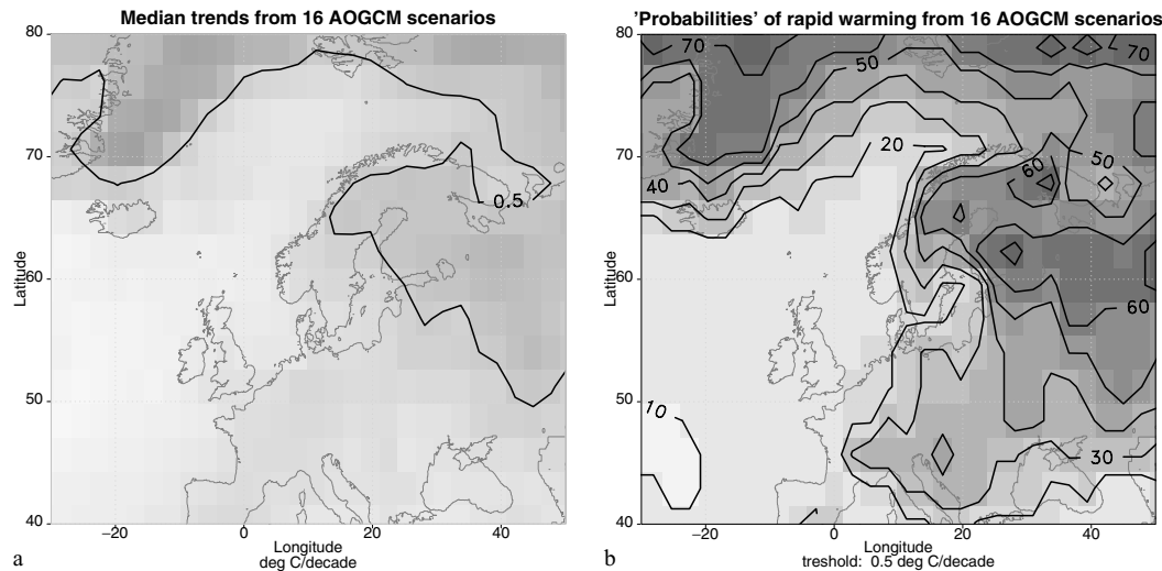
Fig 4. A comparison between the GCM ensemble median linear trend for January 1980–2050 (a) and conditional probability of a warming greater than 0.5\text{ }^{\circ}\text{C decade}^{-1} (b).
