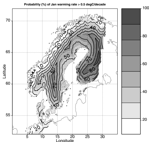
Fig 5. Probability estimates of the warming exceeding a threshold value of 0.5\text{ }^{\circ}\text{C decade}^{-1} in January for “1980”–“2050”, derived from downscaling of the multi-model ensemble and based on the assumption that there is no common systematic bias amongst the various GCMs. The map was produced using the multiple geographical regression model (Table 4) and kriging of the residuals from the geographical model. The stations included in the analysis are marked as black dots.
