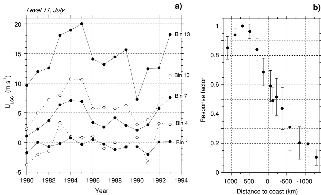
Fig. 4. July mean large-scale zonal wind (model level 11) in selected bins, 1980–1993 (a) and associated response factor (b). Error bars represent one standard error. See text for further explanation.
