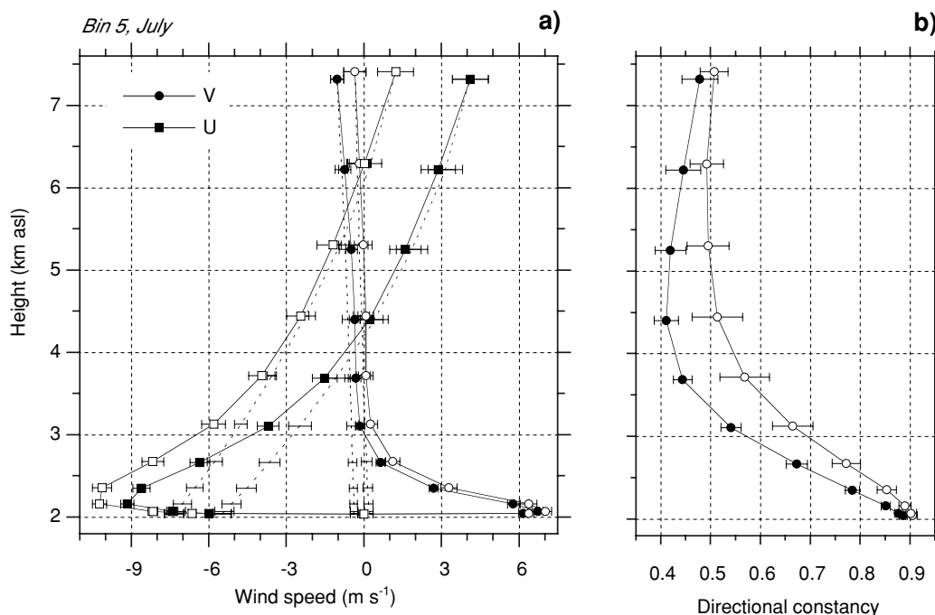
Fig. 6. Bin 5 (1750–2250 m asl), July: average wind components ( U , V ) for strong vortex ensemble (filled symbols) and weak vortex ensemble (open symbols) (a) and directional constancy (b). Dashed lines indicate large scale wind components ( U_{LSC} , V_{LSC} ). Error bars represent one standard error.
