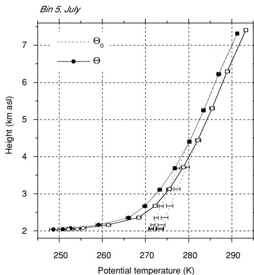
Fig. 5. Bin 5 (1750–2250 m asl), July: average potential temperature \Theta (K) for strong vortex ensemble (filled symbols) and weak vortex ensemble (open symbols). Dashed lines indicate background potential temperature \Theta_0 (K). Error bars represent one standard error.
