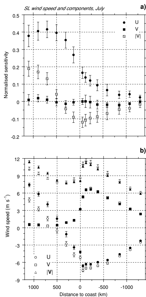
Fig. 10. As Fig. 9, but for SL absolute wind speed and components.
