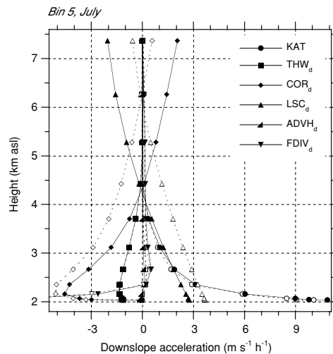
Fig. 7. Bin 5 (1750–2250 m asl), July: average momentum balance terms for strong vortex ensemble (filled symbols) and weak vortex ensemble (open symbols). Error bars represent one standard error.
