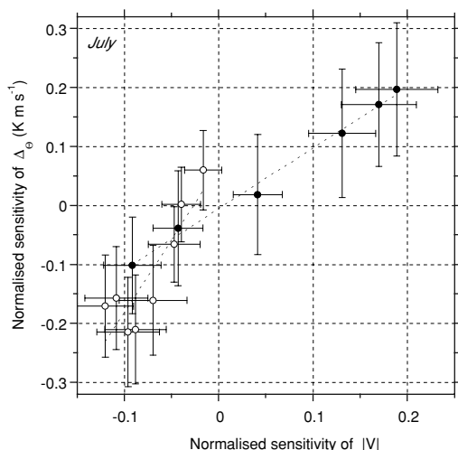
Fig. 13. Normalised sensitivities of surface layer potential temperature deficit \Delta\theta and surface layer wind speed |V| . Open symbols: ice sheet bins; Filled symbols: ocean bins.
