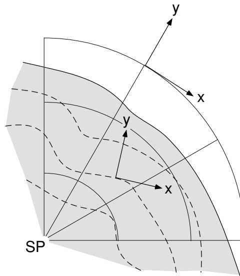
Fig. 3. Orientation of down/cross slope coordinates over the ice sheet (stippled line are schematic height contours) and ordinary W–E and S–N coordinates over the ocean (where slope direction is undefined).
