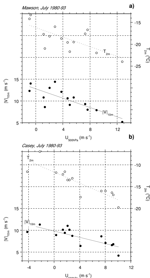
Fig. 2. Observations, July 1980–1993: monthly mean 2 m temperature (open symbols) and 10 m wind speed (filled symbols) as a function of 500 hPa zonal wind, for Mawson (a) and Casey (b).
