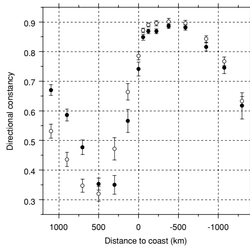
Fig. 11. SL wind directional constancy for strong vortex (open symbols) and weak vortex ensemble (filled symbols).
