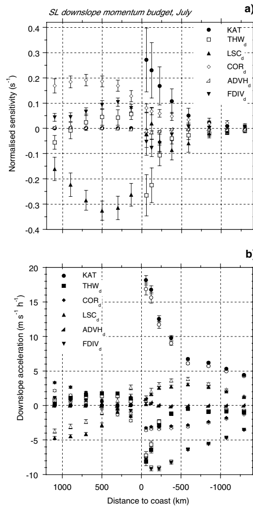
Fig. 12. As Fig. 9, but for SL momentum budget.
