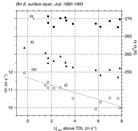
Fig. 8. Bin 8 (150–750 m asl), July, surface layer: correlation of average potential temperature \Theta , background potential temperature \Theta_0 and wind speed |V| with large-scale zonal wind U_{LSC} (model level 11).
