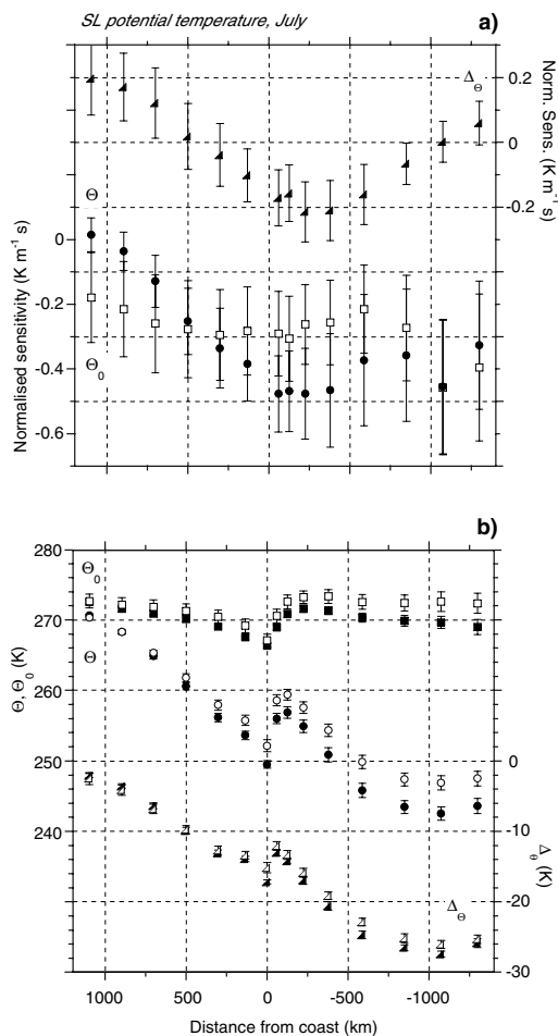
Fig. 9. July, surface layer: (a) normalised sensitivity of SL potential temperature \Theta , background potential temperature \Theta_0 and potential temperature perturbation \Delta\Theta to changes in the zonal large-scale circulation U_{LSC} . Error bars represent one standard error; (b) potential temperature distribution for strong vortex ensemble (filled symbols) and weak vortex ensemble (open symbols).
