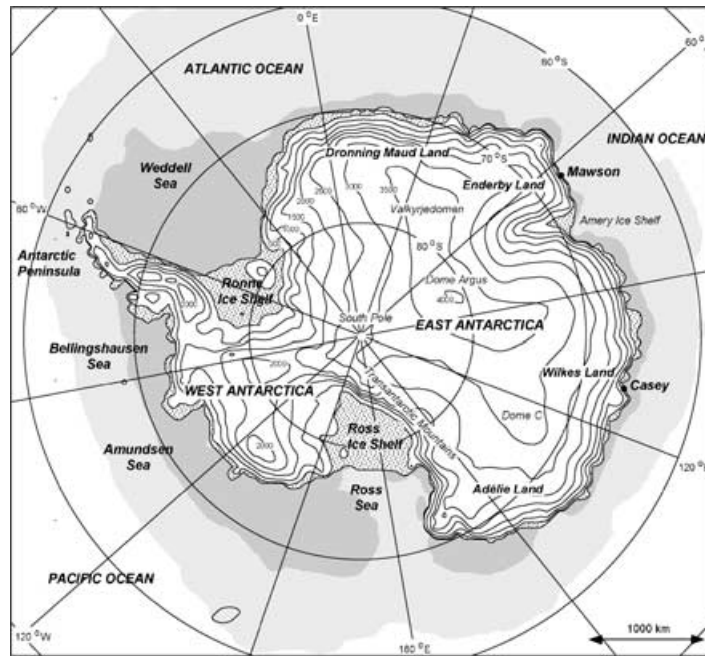
Fig. 1. Model domain and topographical features of Antarctica. Stippled areas, ice shelves, light shaded, average July sea ice extent, dark shaded, average January sea ice extent (from ERA-15). Surface elevation (m asl) is contoured every 500 m.
