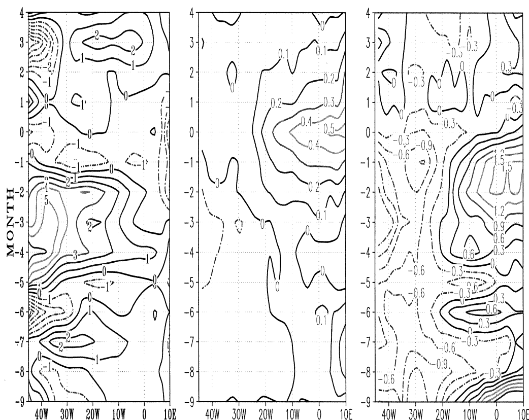
Fig. 4. Hoevmoeller diagram showing the evolution in time of several variables at the equator for the average over the warm events in cluster V. Left: zonal wind anomalies. Center: SST anomalies. Right: heat content anomalies. X-axis: longitude. Y-axis: months after peak.
