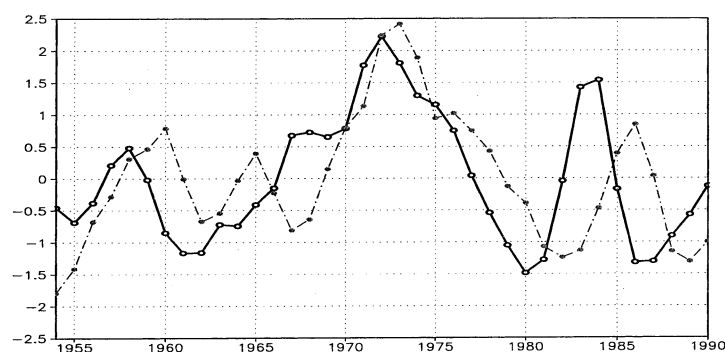
Fig. 1. Reproduction of Fig. 10 in Deser and Blackmon (1993): time series of the second EOF of winter (November–March) SST anomalies (dashed) and SIC anomalies averaged in the Davis Strait–Labrador Sea region (solid). The second EOF of winter SST anomalies explains a 24% of the variance. Both time series have been standardized and detrended.
