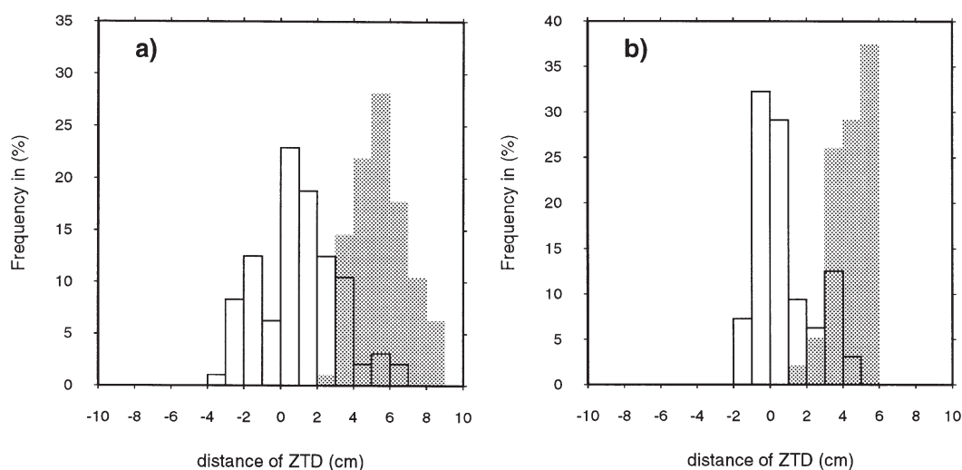
Fig. 3. Frequency distribution of the differences between the GPS-derived ZTD observations and the modeled values (low grid and topography resolutions) at LLIV (grey) and EBRE (white) stations during (a) 14 September 1999 and (b) 10 September 1999.
