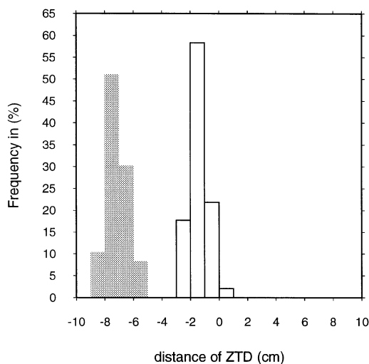
Fig. 4. Frequency distribution of the differences between the GPS-derived ZTD observations and the modeled values at ESCO station during 14 September 1999 using a 5 arcmin topographic and land-use sources (grey) and 30 arcsec topographic and land-use data sets (white).
