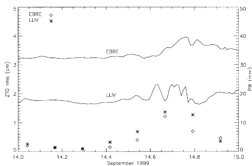
Fig. 2. 3-h interval rms ZTD errors (* LLIV, ◇ EBRE) and modeled precipitable water (continuous line) as a function of time at LLIV and EBRE stations.
