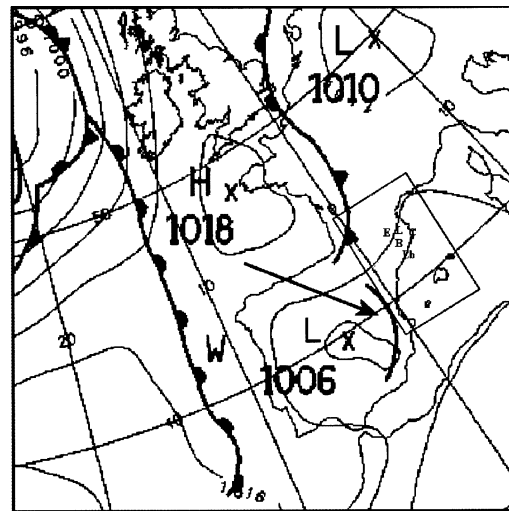
Fig. 1. Surface analysis of the atmospheric flow at 18 UTC 14 September 1999. The arrow indicates the movement of the trough. The geographical location of the GPS sites (E for ESCO, L for LLIV, C for CREU, B for BELL, Eb for EBRE) are indicated at the 6-km grid resolution domain used in the MM5 model. The weather chart has been adapted from a map given by the UK Met-Office.
