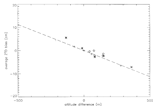
Fig. 5. Comparison of the ZTD differences between the GPS estimates and MM5 modeled values as a function of the altitude increment ( \Delta z ) for 5 arcmin (asterisk), and 30 arcsec (diamond) topographic sources for 14 September 1999. The dashed line ( -0.0225 \Delta z - 0.1348 ) fits the average ZHD differences between the model simulations with the 5 arcmin and 30 arcsec topography sources as a function of the altitude increment, and shows the ZTD variation assuming hydrostatic equilibrium in the atmosphere.
