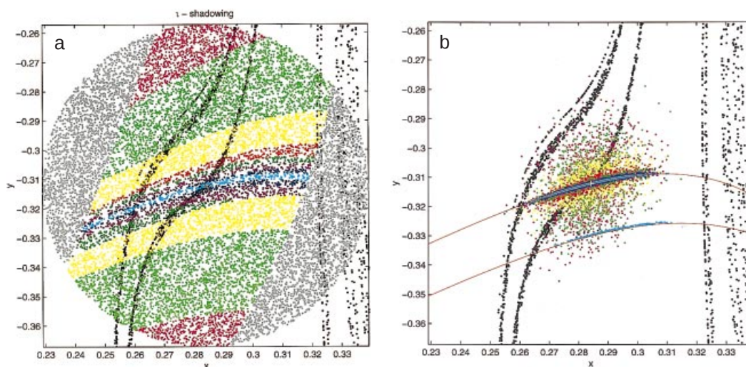
Fig. 2. Noise reduced distributions produced by (a) \iota -shadowing, and (b) 4d-Var. See text for details.
