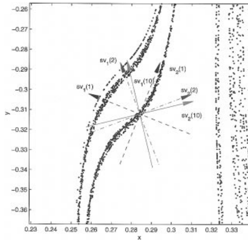
Fig. 3. Orientation of the 1-, 2-, and 10-step initial singular vectors. The orientation of the second one step singular vector sv_2(1) , the shrinking direction, is the same as the orientation of the points which \iota -shadow after one step (Fig. 2a) and the same as the primary orientation of the 4d-Var ensemble for N_a = 1 (Fig. 2b). There is a large degree of rotation between the one step and the two step singular vectors. This accounts for the contraction along the \tilde{W}_s(x^t) seen in both the \iota -shadowing results and the 4d-Var results of Fig. 2.
