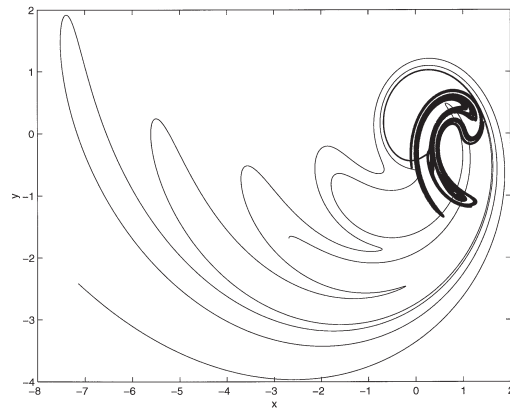
Fig. 1. The Ikeda attractor and the structure of the \tilde{W}_s(\mathbf{x}^t) for the point in Figs. 2, 3. The Ikeda attractor is seen as the dots on the right side of the picture while the \tilde{W}_s(\mathbf{x}^t) is shown as the looping line. The \tilde{W}_s(\mathbf{x}^t) has a rich structure; each time it loops back through the region surrounding the point about which it is constructed it will cause a valley in cost function space.
