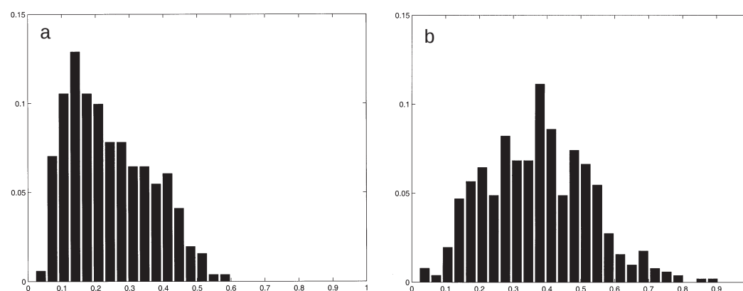
Fig. 5. Distribution of the area containing 90% of the probability in noise reduced analysis PDFs for (a) 4d-Var, and (b) the EnKF over 1024 different initial conditions. The areas are normalised by the area containing 90% of the observational probability. The areas produced by 4d-Var are smaller than those produced by the EnKF, consistent with the 4d-Var ensembles lying along a line given by the \tilde{W}_s(x^t) while the EnKF ensembles reflect the underlying attractor structure. The combination of the 4d-Var and EnKF PDFs results in an improvement of nearly two orders of magnitude. Although the histogram is not shown, all areas of the combined results would fall into the first bin of panels (a) and (b).
