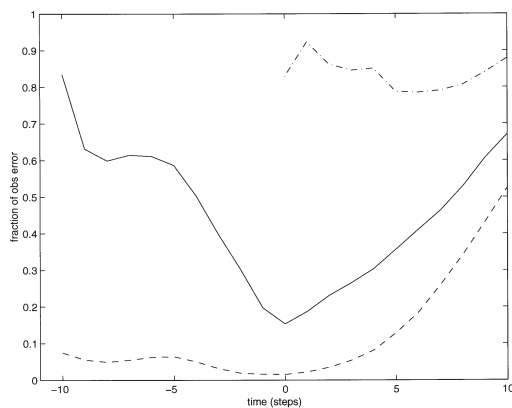
Fig. 6. Mean distance between the ensemble mean and truth for N_a = 10 4d-Var ensembles (solid), the EnKF Ensembles (dot-dashed), and the combined 4d-Var/EnKF ensembles (dashed) over 1024 different initial conditions. Analysis ensembles for 4d-Var and combined 4d-Var/EnKF were constructed and integrated forward 20 steps. The first 10 steps covered the assimilation window, with the next 10 steps being proper predictions. As the EnKF ensembles do not utilise a “window” they were integrated over only the 10 forecast steps. All errors are normalised by the error that results from performing no noise reduction and simply constructing an ensemble about an observation. It is seen that the combined ensemble outperforms the 4d-Var ensemble at every step.
