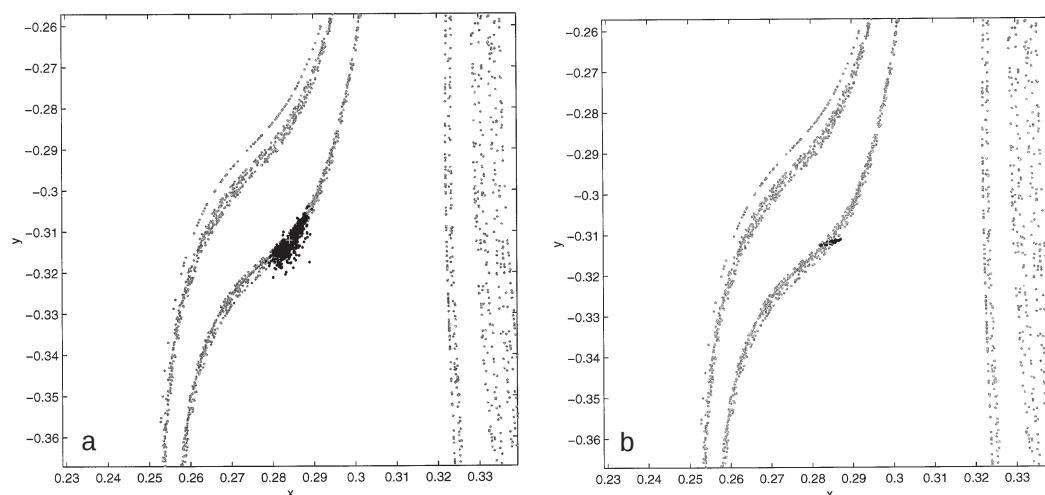
Fig. 4. Noise reduced distributions produced by (a) the EnKF and (b) the combination of the N_a = 10 4d-Var PDF (Fig. 2b) and the EnKF PDF. In both panels, the grey dots are points on the Ikeda attractor.
