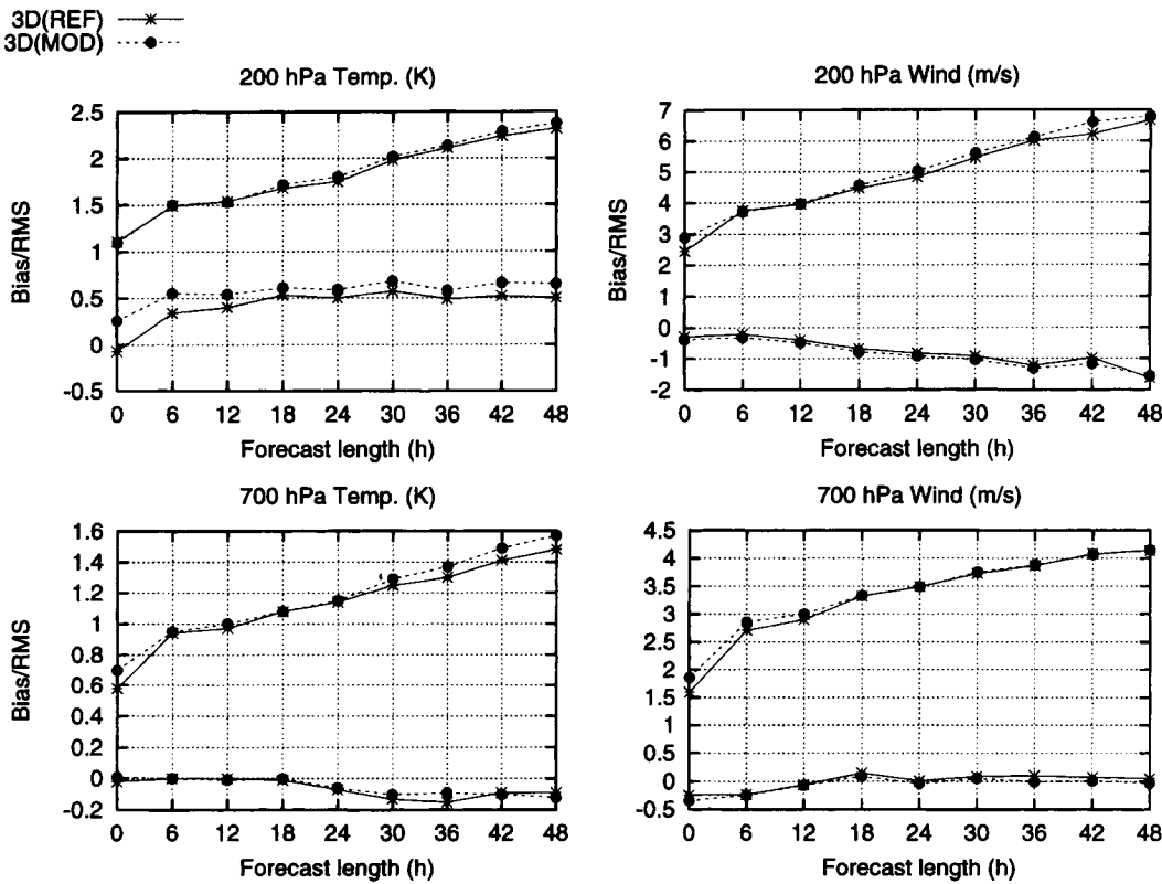
Fig. 9. Average bias and rms scores for the first week of the winter period (10–16 February 1998), as functions of forecast length (h). Temperature scores (K) at 700 hPa (lower left) and 200 hPa (upper left) as well as wind speed scores (m/s) at 700 hPa (lower right) and 200 hPa (upper right). The scores are for the reference spectral 3D-Var run (full) with all significant level data used and for the modified run (dashed) with only standard pressure level data from TEMP and PILOT pressure level reports used.
