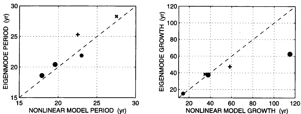
Fig. 10. Comparison of oscillations period and growth rate for the unstable eigenmode and the nonlinear model for different vertical diffusivities K_v = 10^{-4} (+) and 0.5 \times 10^{-4} (x) \text{m}^2 \text{s}^{-1} , with (O) and without wind forcing (zonal windstress according to Bryan, 1987). Also represented (*) is the result from a model of higher resolution ( 32 \times 28 horizontally, 15 levels vertically) for K_v = 10^{-4} \text{m}^2 \text{s}^{-1} and no wind forcing.
