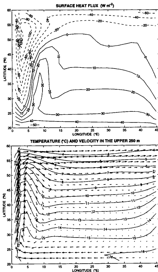
Fig. 1. (a) Surface heat flux ( \text{W m}^{-2} ) diagnosed at year 1000 of the model simulation under restoring boundary conditions with a constant \gamma = 35 \text{ W m}^{-2} \text{ K}^{-1} to a linear profile of temperature, zonally uniform and linearly varying with latitude from 25^\circ\text{C} at 20^\circ\text{N} to 2^\circ\text{C} at 60^\circ\text{N} . (b) Upper 250 m temperature ( ^\circ\text{C} ) and velocities ( 0.5 \text{ cm/s} per degree).
