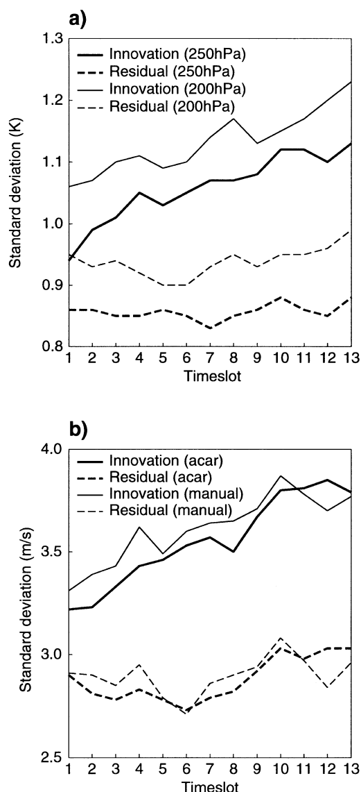
Fig. 6. Standard deviation of innovations (solid lines) and residuals (dashed lines) in 4D-Var for AIREP temperature at 200 hPa and 250 hPa (a), and for AIREP component wind separately for two different kind of aircraft reports (manual and acar) at 250 hPa (b) over North America in an assimilation experiment with a 12 h assimilation window. The curves are based on innovation and residual sequences from 16 September to 10 October 1998.
