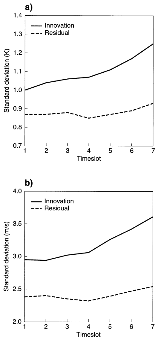
Fig. 4. Standard deviation of innovations (solid lines) and residuals (dashed lines) in 4D-Var for AIREP (amdar) temperature (a) and AIREP (acar) component wind (b) at 250 hPa over the North Atlantic. The curves are based on innovation and residual sequences from 16 to 29 April 1998. Amdar and acar are two slightly different aircraft observation reporting systems.
