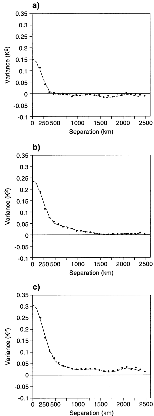
Fig. 1. A discretized representation of a probability distribution function of innovation covariances for a 30 min timeslot 1 (a), for 1 h timeslot 4 (b) and for 1 h timeslot 6 (c) for AIREP temperature over North America at 200 hPa. The 4D-Var innovation sequence is from 1 September 1997 to 15 October 1997.
