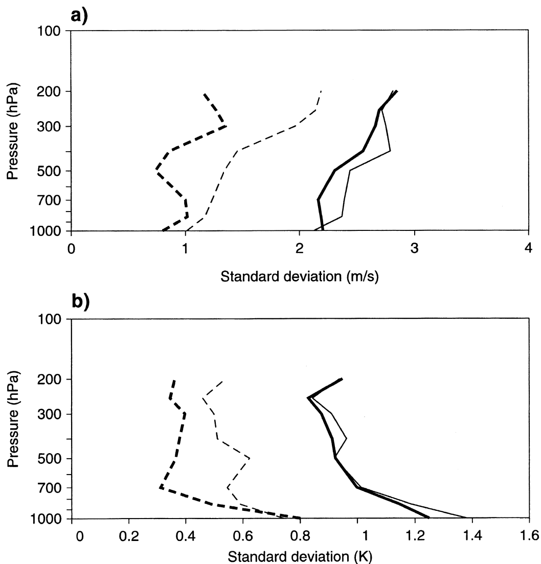
Fig. 3. Vertical profiles of the background (dashed line) and observation (solid line) error standard deviation at the beginning (thick line) and at the end (thin line) of the 6-h assimilation window for AIREP component wind (a) and temperature (b) over North America. The 4D-Var innovation sequence is from 1 September 1997 to 15 October 1997.
