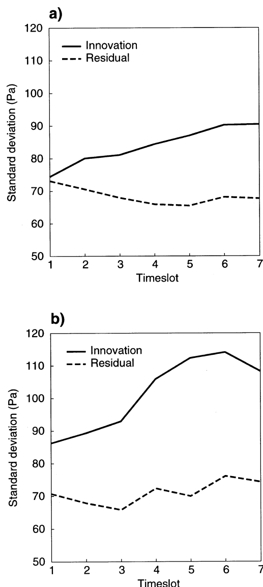
Fig. 5. Standard deviation of innovations (solid lines) and residuals (dashed lines) in 4D-Var for DRIBU surface pressure in the North Atlantic (a) and in the South Atlantic (b). The curves are based on innovation and residual sequences from 16 to 29 April 1998.
