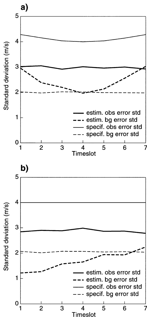
Fig. 2. Estimated (thick lines) and specified (thin lines) standard deviation of background error (dashed lines) and observation error (solid lines) in 3D-Var (a) and in 4D-Var (b), respectively, for AIREP component wind over North America at 200 hPa. The estimation is based on an innovation sequence from 1 September 1997 to 15 October 1997. The numbering of timeslots is as follows. Timeslot 1 (7) cover the first (last) 30 min of the 6-h assimilation window. 1 h timeslots 2–6 are centered around full hours of the window. Timeslot around 12UTC, for instance, is number 4.
