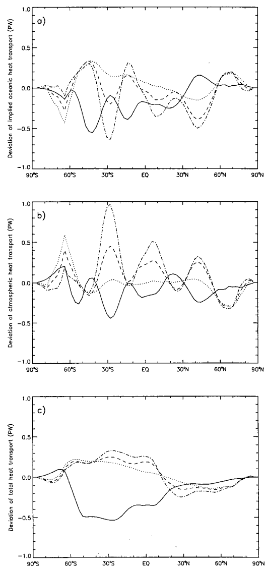
Fig. 5. Annual-mean, meridional heat transport (in PW) averaged over nine years for the different experiments, shown as deviations from the control case. -5X (solid), 1X (dotted), 5X (dashed), 9X (dot-dashed). (a) Implied oceanic heat transport deviations. (b) Atmospheric heat transport deviations. (c) Total heat transport deviations.
