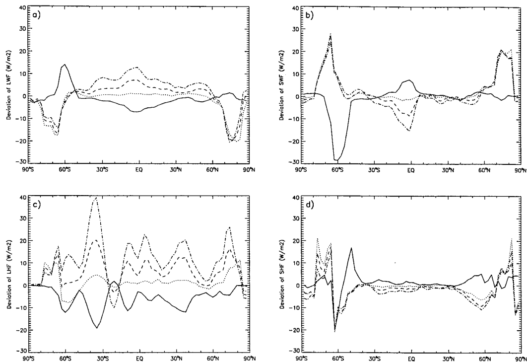
Fig. 8. Same as Fig. 7 except for vertical energy flux at the surface. (a) Deviations of downward longwave radiation (LWF) from 0X. (b) Deviations of downward shortwave radiation (SWF) from 0X. (c) Deviations of the latent heat flux (LHF) from 0X. (d) Deviations of the sensible heat flux (SHF) from 0X.
