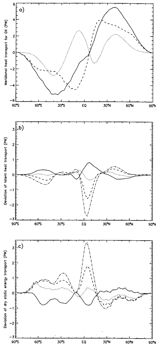
Fig. 6. (a) Meridional transport (in PW) of moist static energy (solid), dry static energy (dashed) and latent heat (dotted) for the annual mean of year 3 of the control case (0X). (b) Deviations from 0X of meridional latent heat transport for the year-3, annual mean, -5X (solid), 1X (dotted), 5X (dashed), 9X (dot-dashed). (c) Same as (b) except deviations from 0X of dry static energy transport.
