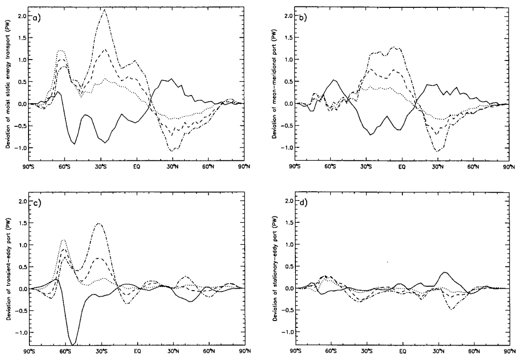
Fig. 12. Same as Fig. 10 except for JJA mean.
