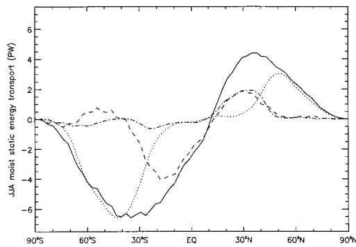
Fig. 11. Same as Fig. 9 except for JJA mean.
