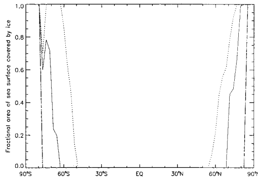
Fig. 2. Fractional area of the ocean surface that is covered by sea ice in the annual mean as a function of latitude. 0X (solid); -5X (dotted); 1X, 5X and 9X (dashed).
