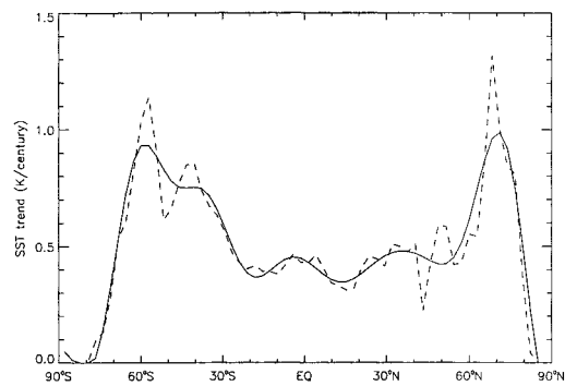
Fig. 1. Least-square trend in annual-mean, zonally averaged sea surface temperature (in K per century) from GISST2 data as a function of latitude. The dashed curve represents the raw data. The solid curve represents the data after spatial smoothing.
