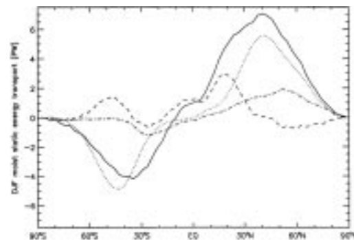
Fig. 9. DJF-mean moist static energy transport (solid), averaged over ten years for the control case (in PW); decomposed into mean-meridional part (dashed), stationary-eddy part (dot-dashed) and transient-eddy part (dotted).
