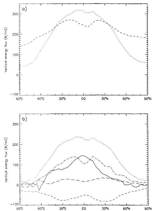
Fig. 3. Zonally averaged, annual-mean vertical energy flux ( \text{W m}^{-2} ) averaged over ten years of the control case (0X) as a function of latitude. (a) At the top of the atmosphere OLR (dashed) and ASR (dotted). (b) At the surface downward shortwave radiation (SWF, dotted), latent heat flux (LHF, dot-dashed), downward longwave radiation (LWF, dashed), sensible heat flux (SHF, long dashes), net downward surface energy flux (solid).
