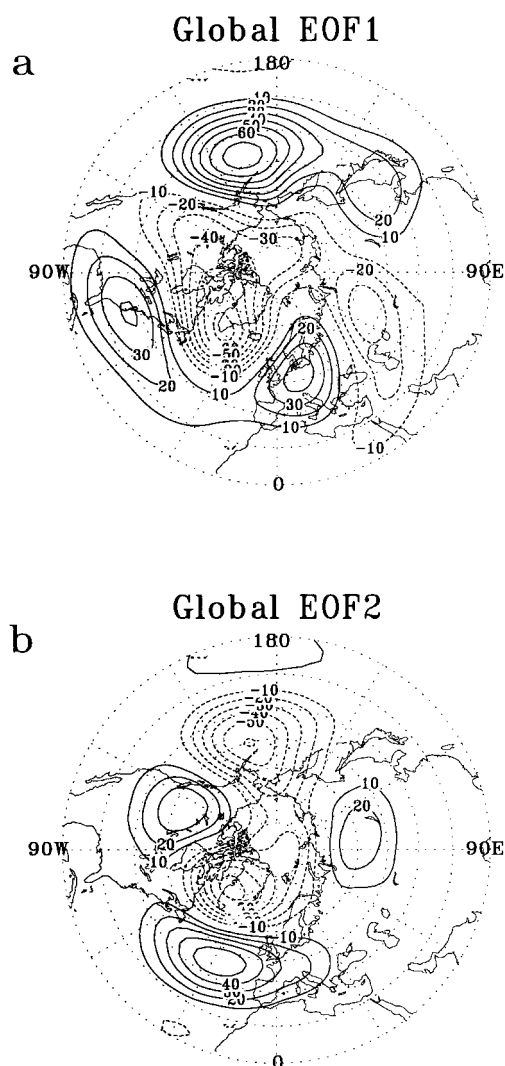
Fig. 7. (a) First 500 hPa geopotential EOF monthly anomaly during winter (DJF) from NMC analysis data. (b) As in (a) but for the second EOF. Contour interval 10m. Negative values are dashed.
