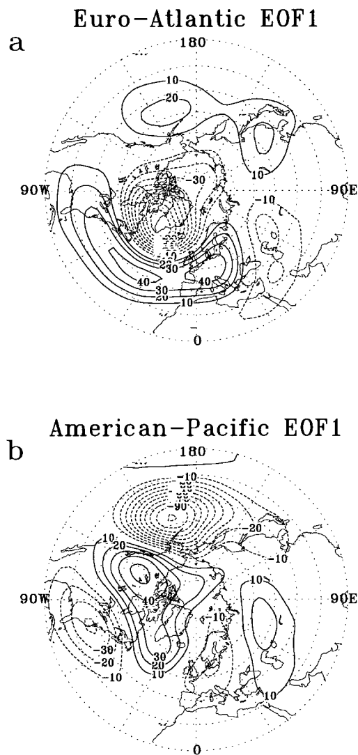
Fig. 2. (a) First 500 hPa geopotential height Euro-Atlantic EOF (monthly anomalies) for winter (DJF) from NMC analysis data. (b) as in (a) but for the first American-Pacific EOF. Contour interval 10m. Negative values are dashed.
