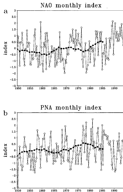
Fig. 3. Time series of the principal components of the two dominant empirical orthogonal functions of 500-hPa monthly-mean observed geopotential height over the northern hemisphere for the period 1949–1994. (a) Euro-Atlantic sector; (b) American-Pacific sector. Open circles: monthly time series; solid circles: 10-year running means of the monthly series.
