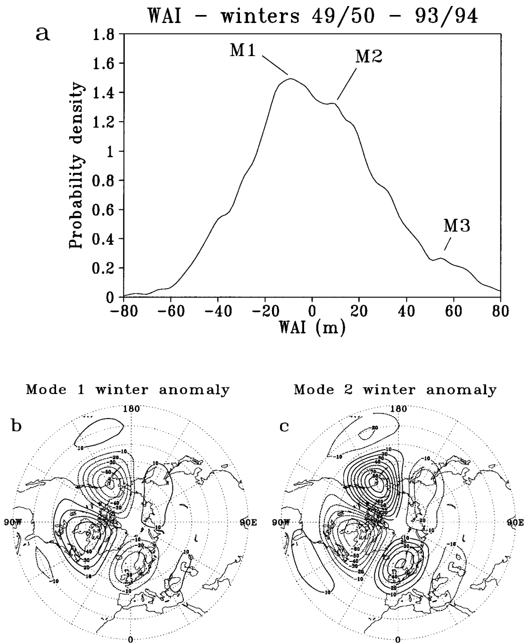
Fig. 4. (a) Probability density estimation of the WAI computed in the [45^{\circ}\text{N}-70^{\circ}\text{N}] zone from the winters 1949–1994. (b) and (c) Mode 1 and Mode 2 composites (see text). Contour interval 10m. Negative values are dashed.
