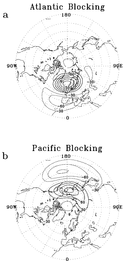
Fig. 1. “Blocking signature” (i.e., the difference of blocked and zonal days ensemble means) for the Euro-Atlantic (a) and Pacific (b) blocking in the December–February period. Contour interval 30\text{m} . Negative values are dashed.
