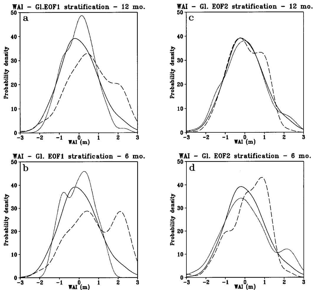
Fig. 8. WAI probability density functions, stratified by the sign of global EOF1 and EOF2. (a) 12-month samples having the highest (positive and negative) values of the EOF1 index; (b) as (a) but for 6-month samples; (c) 12-month samples having the highest (positive and negative) values of the EOF2 index; (d) as (c) but for 6-month samples. Solid line: control climate; dashed line: positive values; dotted line: negative values.
