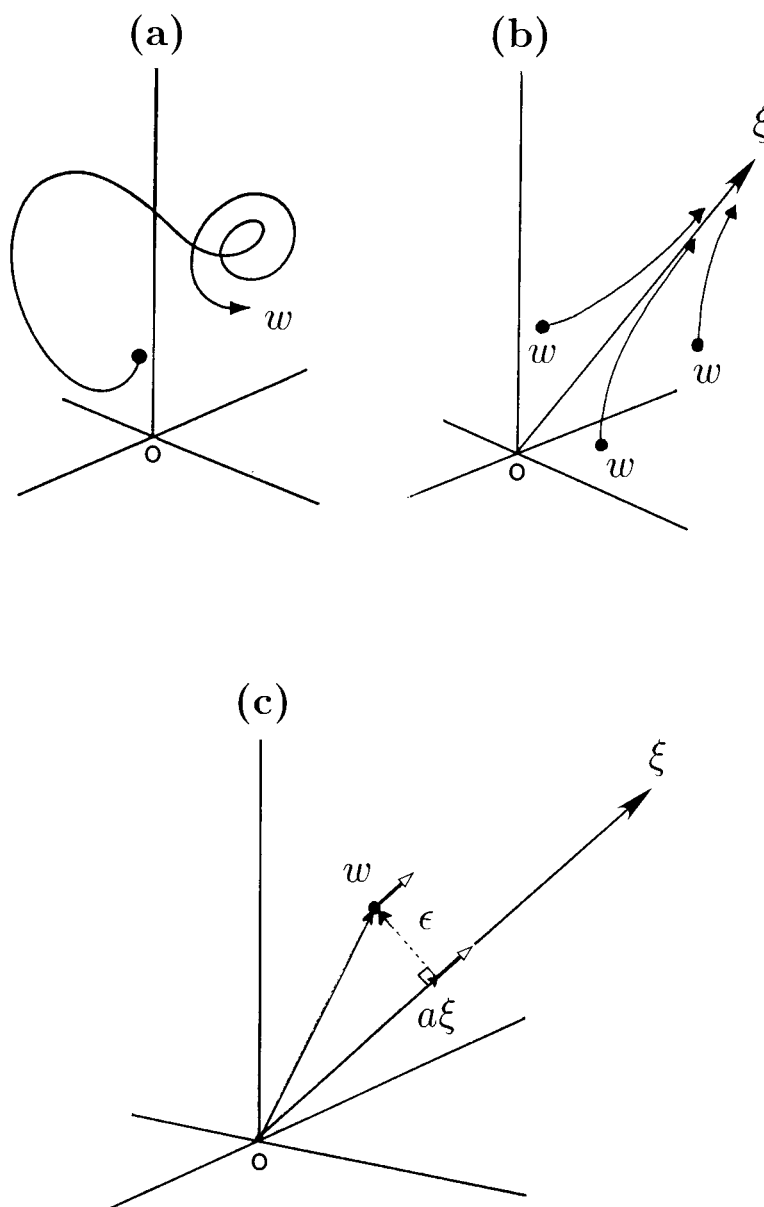
Fig. 4. Schematic illustration of a time evolution of the solution trajectory W in a phase space (a) for the nonlinear system (4); (b) for the unstable linear system (6); and (c) for the orthogonal projection of W onto the unstable direction \xi (16).
