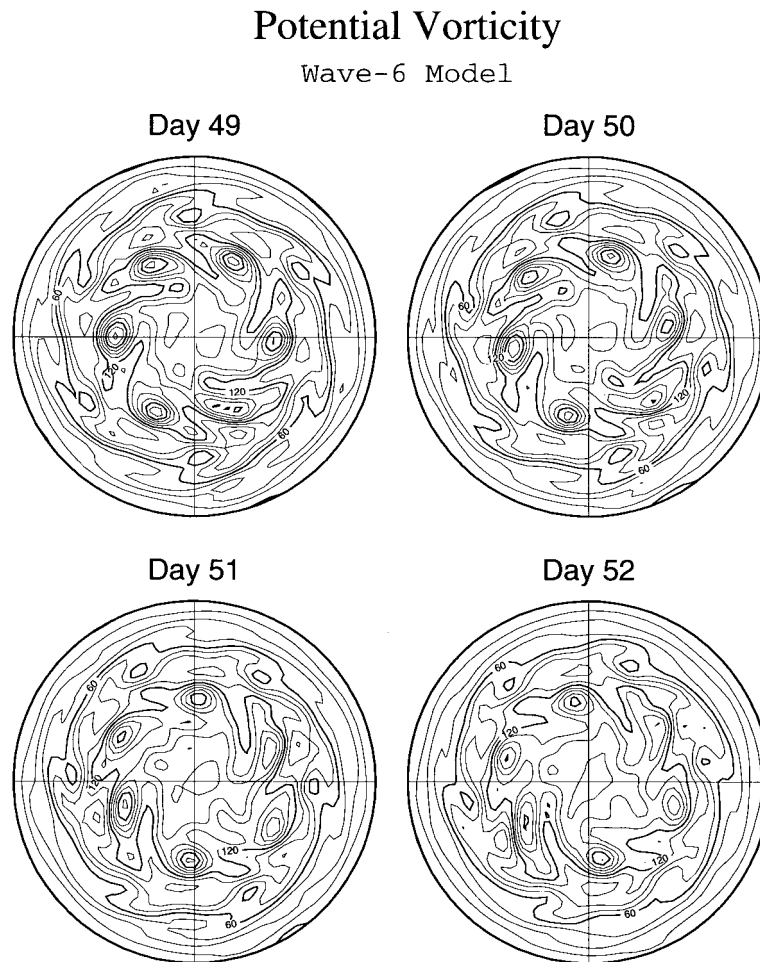
Fig. 9. As in Fig. 6, but for the experiment run with 1.3 times the growth rate for days 49 through 52 when the first wave-breaking occurs.
