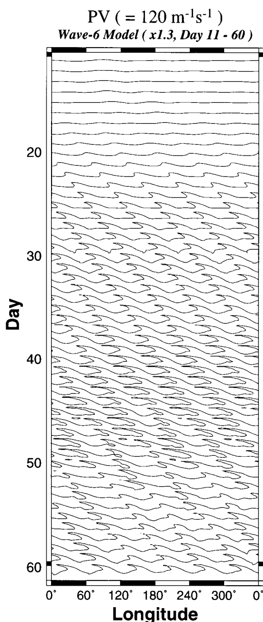
Fig. 10. Schematic illustration of breaking Rossby waves expressed by the contours of 120 PV in Fig. 9 as functions of time (day) and longitude.
