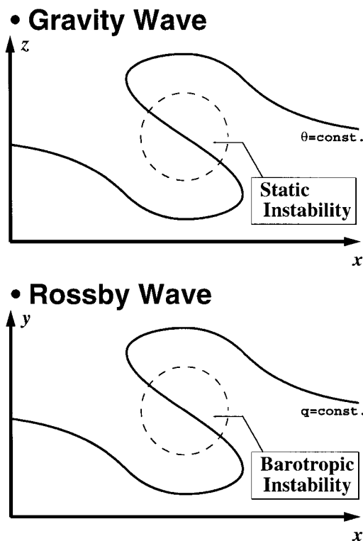
Fig. 3. Schematic illustration of gravity wave breaking in the vertical section (upper) and Rossby wave breaking in the meridional section (lower).
