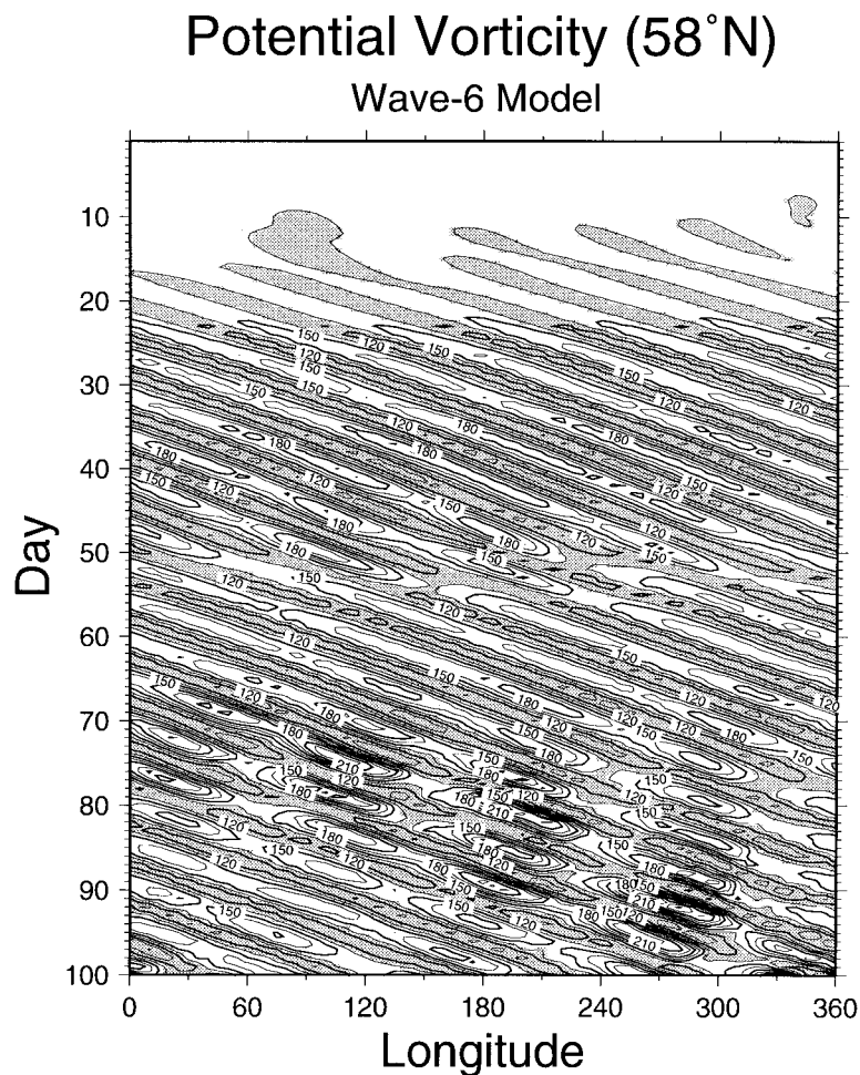
Fig. 8. As in Fig. 7, but for the experiment run with 1.3 times the growth rate during the first 100 days.
