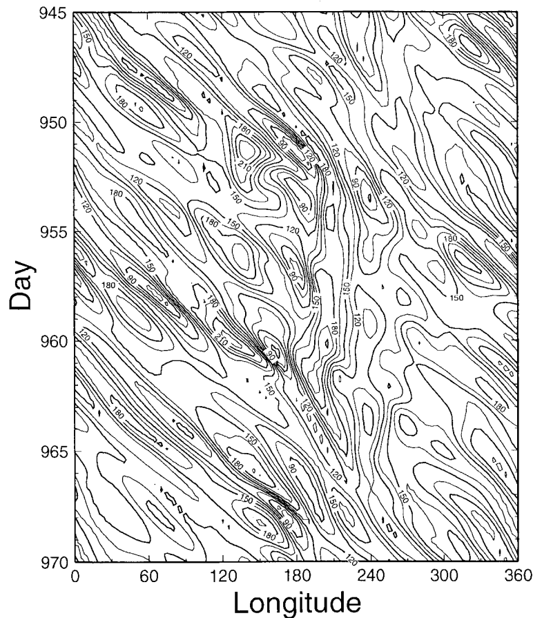
Fig. 2. Longitude–time series of potential vorticity along 58^\circ\text{N} for a life-cycle of a blocking in the barotropic model atmosphere. The units are 10^{-10} \text{ m}^{-1} \text{ s}^{-1} (after Tanaka, 1998).
