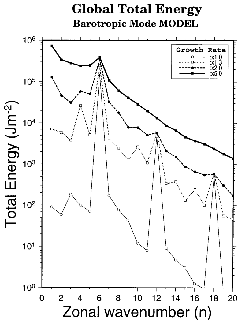
Fig. 13. Mean energy spectra over the zonal wavenumber domain for the wave-6 model during days 30 to 100 with various magnification for the growth rates.
