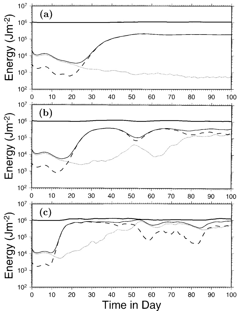
Fig. 14. Time series of total energy in the zonal (thick solid line) and eddy (thin solid line) components during the first 100 days. The eddy components are further divided in the sum of harmonic waves of n = 6, 12 , and 18 (dashed line) and the rest of the non-harmonic waves (dotted line). (a) for the control run; (b) for the 1.3 times the growth rate; and (c) for the doubled-growth rate, respectively.
