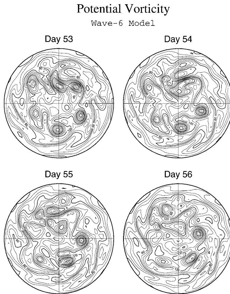
Fig. 12. As in Fig. 6, but for the experiment run with doubled growth rate for days 53 through 56.
