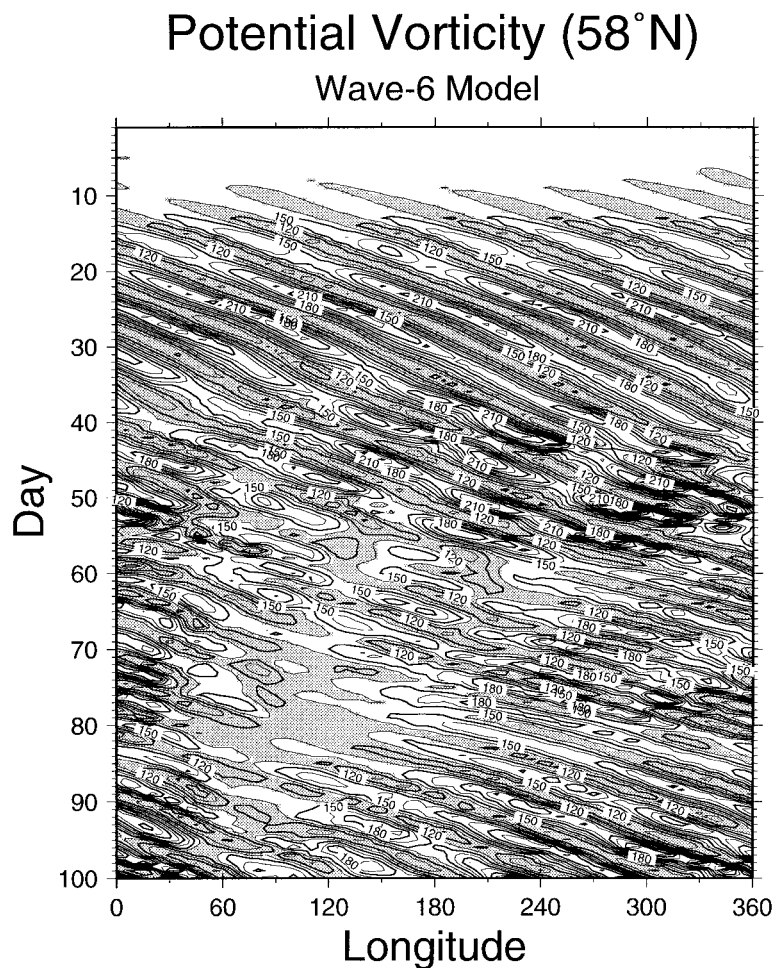
Fig. 11. As in Fig. 7, but for the experiment run with the doubled growth rate.
