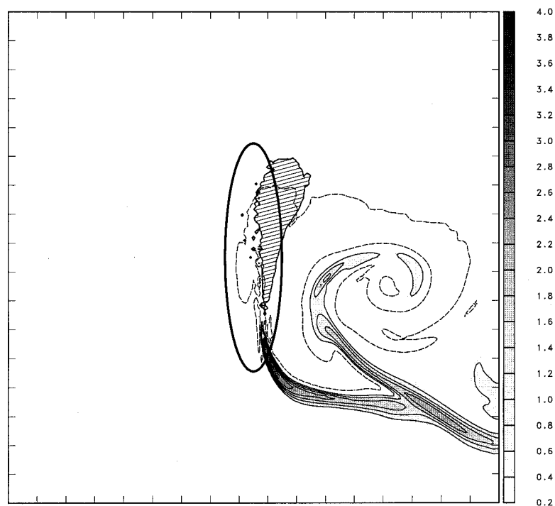
Fig. 5. Perturbation potential vorticity field at the 10-m level. The contour interval is 0.5 pvu ( 1 \text{ pvu} = 10^{-6} \text{ K m}^2 \text{ s}^{-1} \text{ kg}^{-1} ). The region where the turbulent dissipation is active is represented by the hatching. The tick mark spacing on the boundary represents a distance of 300 km (10 grid intervals). The 750-m terrain contour ( h/4 ) is shown by the bold ellipse.
