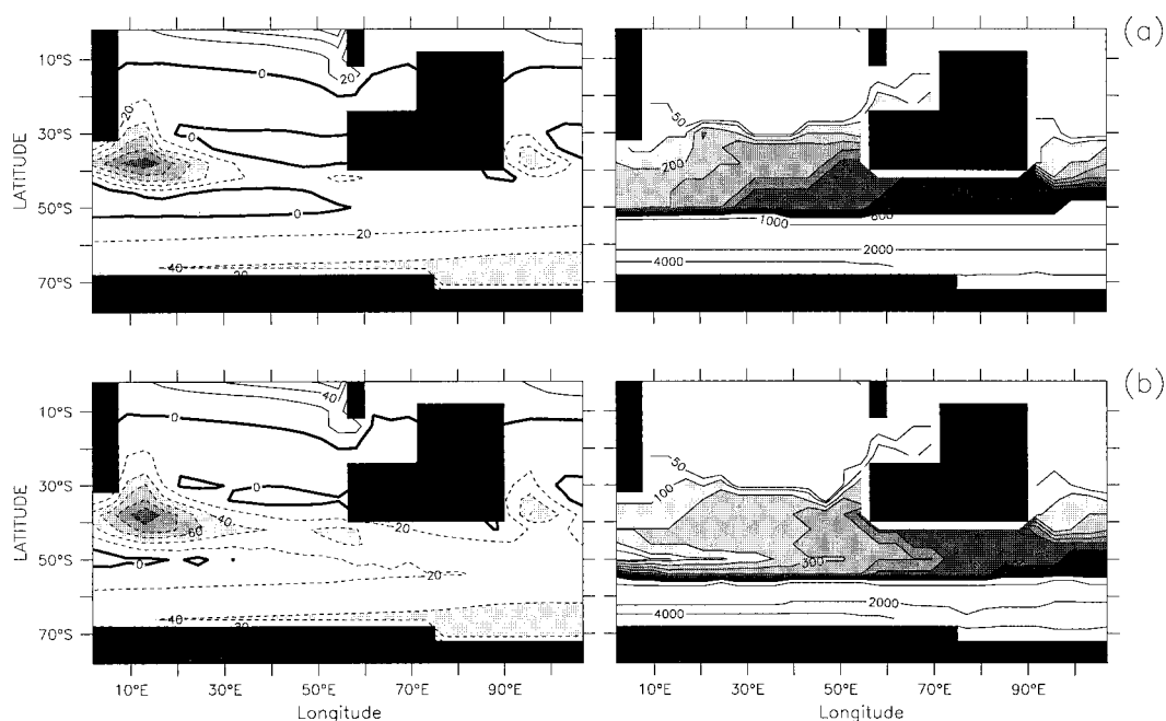
Fig. 4. Results from the first set of short termed integrations initialized with output from the first control experiment: (a) heat fluxes ( \text{W m}^{-2} ) (left panel), and depth of convection (m) (right panel) of the enhanced wind experiment; (b) heat fluxes ( \text{W m}^{-2} ) (left panel), and depth of convection (m) (right panel) of the weakened wind experiment. Contours and shading as in Fig. 1.
