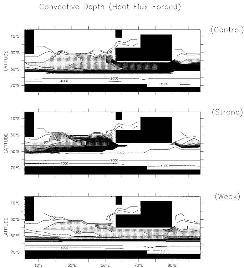
Fig. 5. Results from the second set of short term integrations initialized with output from the first control experiment. Shown is the depth of convection (m) computed during the: (a) control, (b) enhanced, and (c) weakened wind experiment. In all integrations, only salinity was restored to Levitus data. Heat fluxes were diagnosed from the first control experiment and used instead of temperature forcing.
