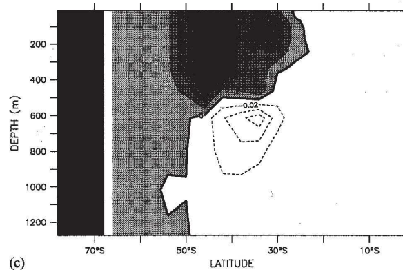
Fig. 6. (a) Temperature, (b) salinity, and (c) density ( \sigma_t ) anomalies computed as the difference between the enhanced wind experiment ( 2 \times \text{HR} ) and the first control run. Anomalies within the SAMW depth range have been shaded. Contour intervals are 0.1^\circ\text{C} for temperature, 0.01 for salinity, and 0.01 \text{ kg m}^{-3} for density.
