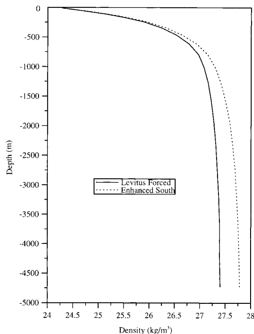
Fig. 3. Mean density profile computed for the south Indian Ocean basin only. Data for both profiles are from the 1st and 2nd control experiments.
