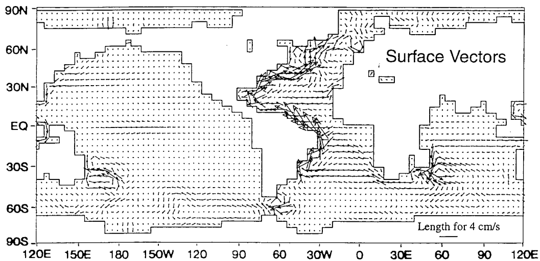
Fig. 5. Vector difference in surface currents between the control and perturbed integrations (i.e., the states I and II) of the standard version of the coupled ocean-atmosphere model. The difference vectors represent the time means over years 5901–6000 of both integrations.
