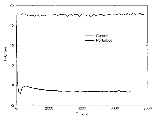
Fig. 3. Time series of 100-year mean intensity of the THC (in units of Sverdrups, i.e., 10^6 \text{ m}^3 \text{ s}^{-1} ) in the North Atlantic Ocean. Thin line: control integration. Thick line: perturbed integration. The intensity of the THC is defined as the maximum value of the streamfunction of meridional overturning circulation.
