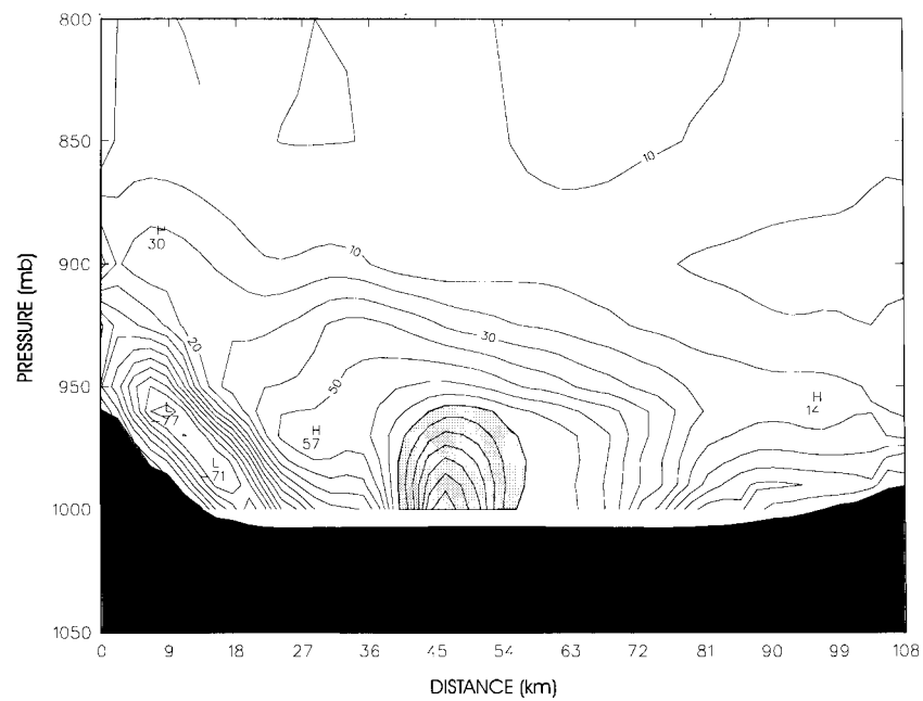
Fig. 8. MM5 simulation. Vorticity east-west cross-section through the vortex at 0600 UTC in the nested domain. Contour interval is 10 units. Shading is for values exceeding 80 \times 10^{-5} \text{ s}^{-1} .
