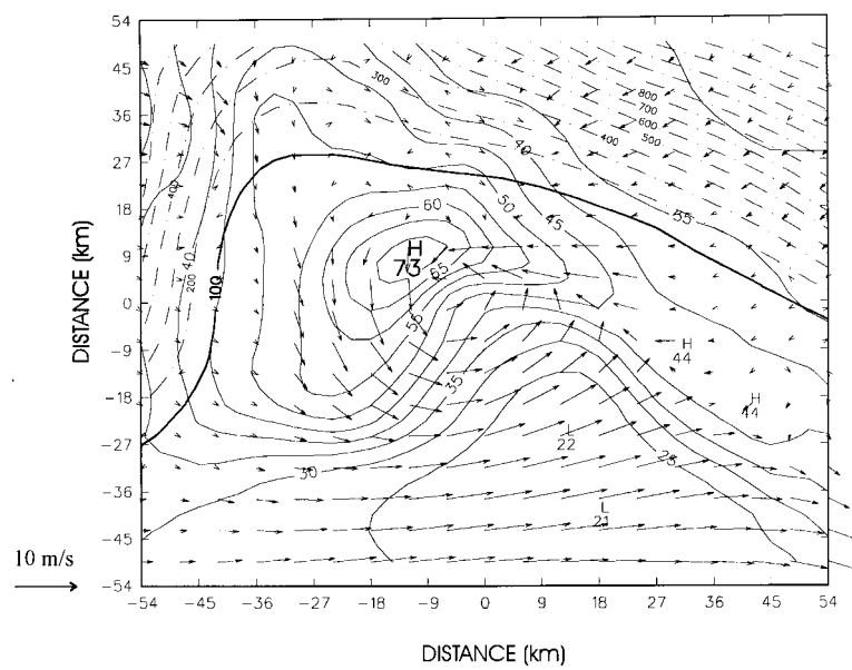
Fig. 9. MM5 simulation. Nested domain winds and relative humidities at 0600 UTC at the altitude of about 50 m above mean sea level. Relative humidity contour interval is 5%. Topography is indicated by dashed lines with 100 m interval.
