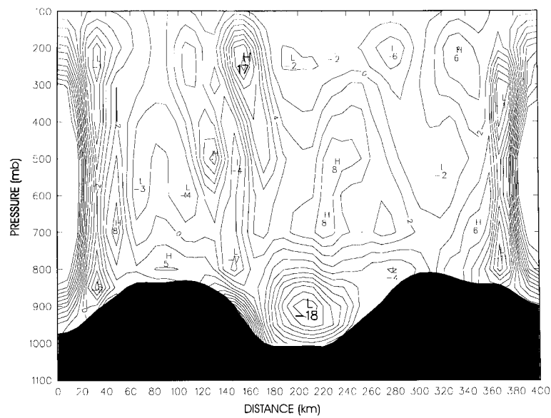
Fig. 10. MM4 simulation. East-west cross section of \omega (Pa/s) at 0300 UTC with a contour interval of 2 \text{ Pa s}^{-1} ( +2 \text{ Pa s}^{-1} \sim -0.2 \text{ m s}^{-1} ). Lateral boundaries disturbances can be noticed.
