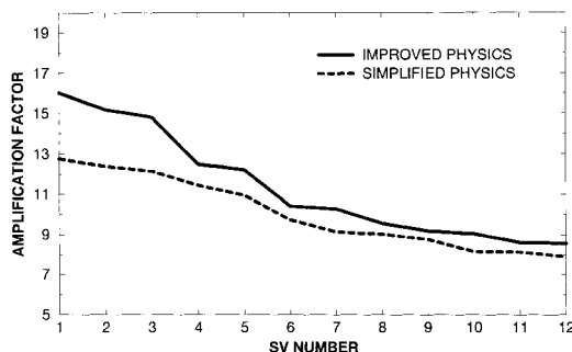
Fig. 10. Spectrum of the first 12 singular vectors computed with a T42L31 linearized model including simplified physics (dashed line) and improved physics (solid line). Singular vectors are optimized over a 48-h period above 30 N.
