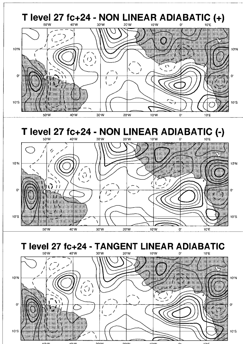
Fig. 4. Same as Fig. 1 but over the tropical Atlantic.
