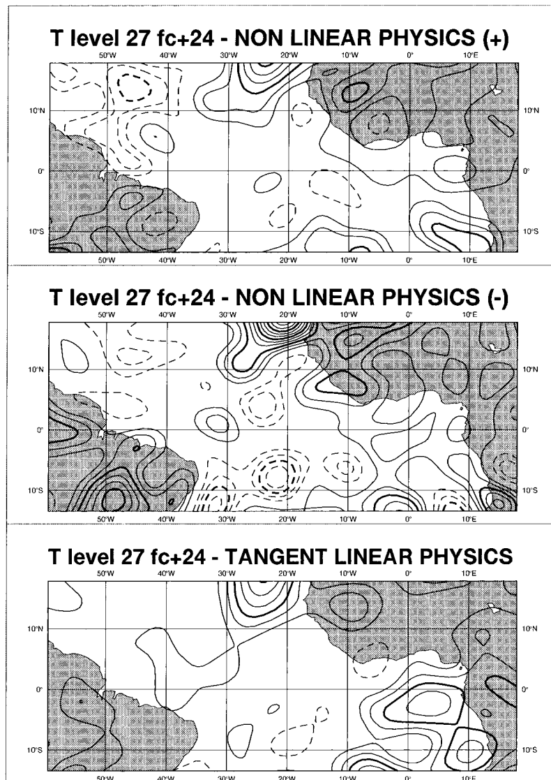
Fig. 5. Same as Fig. 2 but over the tropical Atlantic.
