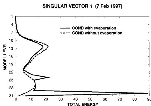
Fig. 9. Influence of rainfall evaporation on the total energy profile of the first singular vector after a 48-h tangent-linear evolution starting on 7 February 1997. The solid line represents the vertical profile when evaporation of rainfall is taken into account in the linearized large-scale condensation parametrization, and the dashed line the vertical profile when evaporation of rainfall is strongly reduced.
