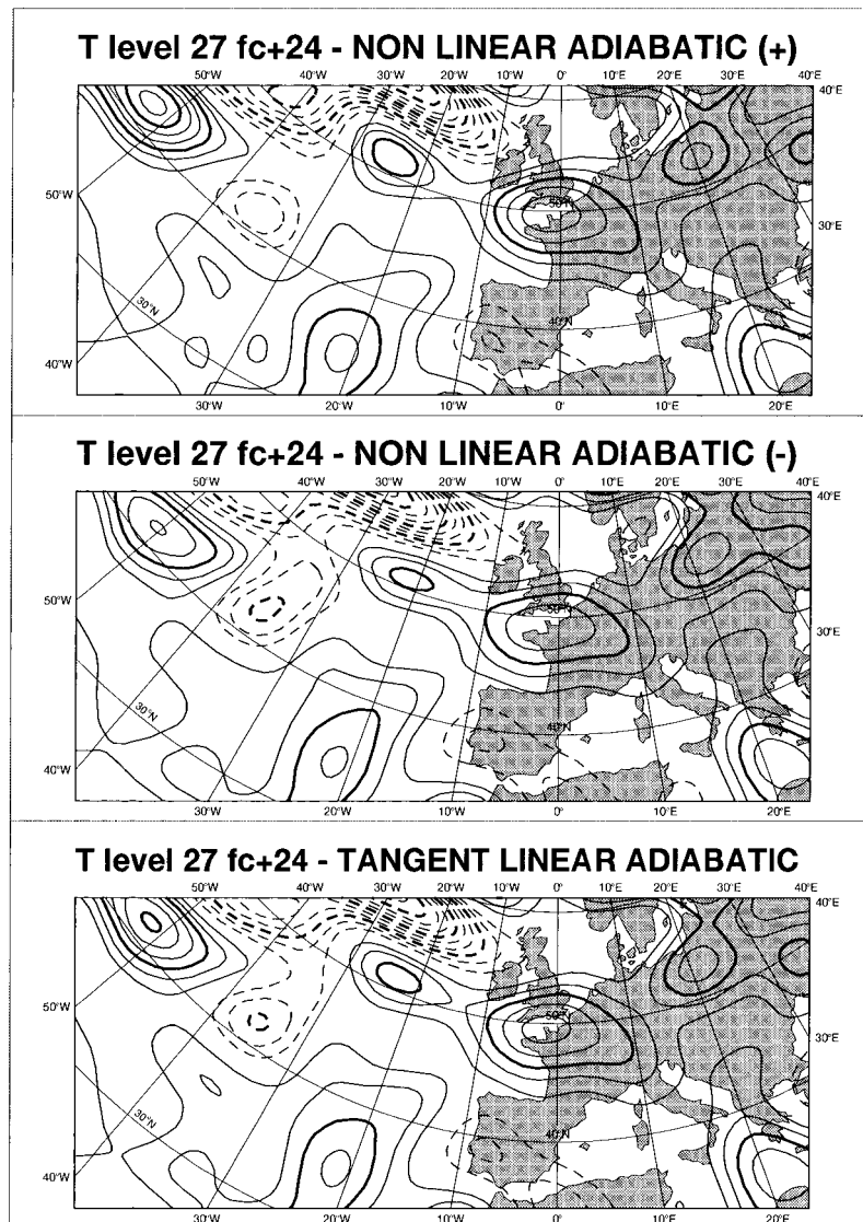
Fig. 1. 24-h evolution of temperature analysis increments at level 27 produced from the difference between two adiabatic non-linear integrations (upper and middle panels) and from an adiabatic tangent-linear integration (lower panel) over Western Europe. Initial perturbations of opposite signs are evolved in the two non-linear integrations. The opposite sign of the result is presented in the middle panel for a direct comparison with the upper panel. Contours are plotted every 0.25 K with negative values in dashed.
