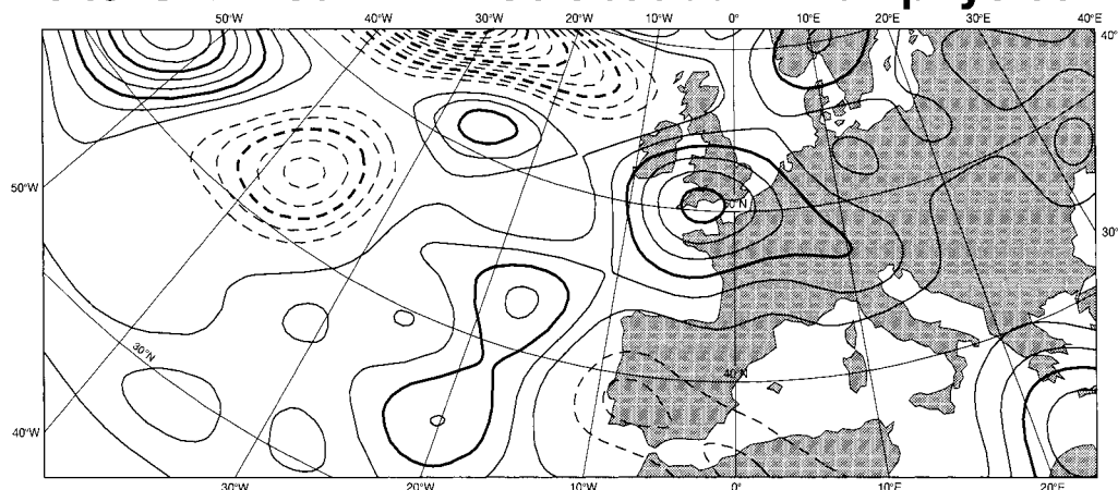
Fig. 3. Same as Fig. 1 (lower panel corresponding to the tangent-linear evolution) but where the increments are evolved with an adiabatic tangent-linear model around a trajectory computed with full physics.
