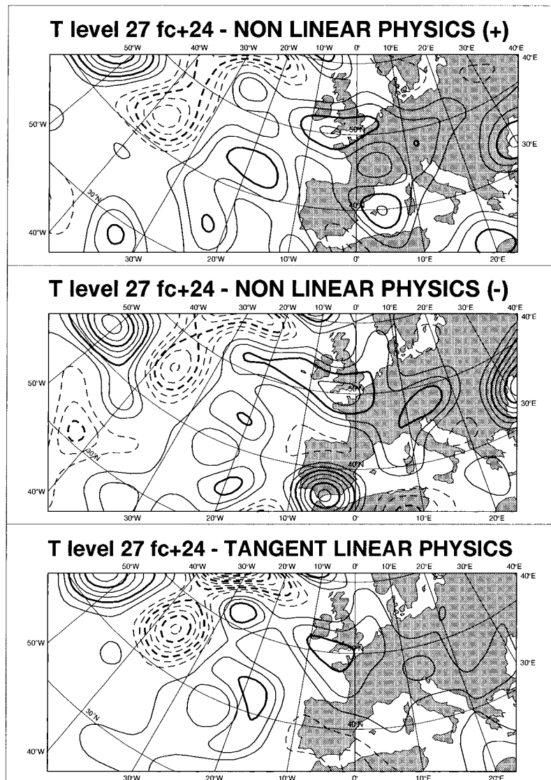
Fig. 2. Same as Fig. 1, but for non-linear and tangent-linear integrations including physical processes.
